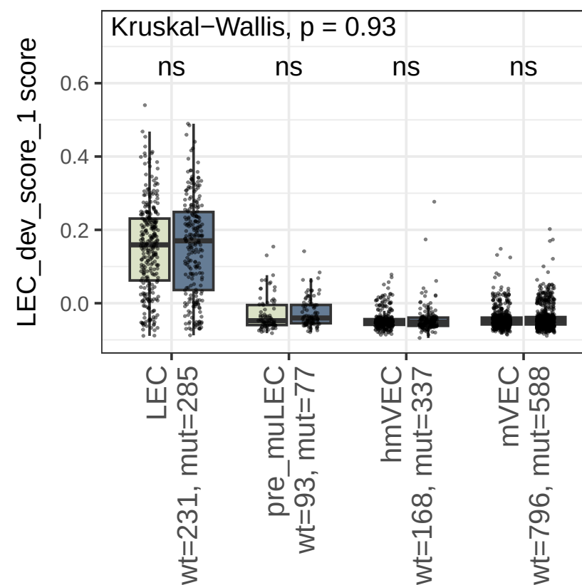
LEC_dev_score_1, RAW PVALUE
