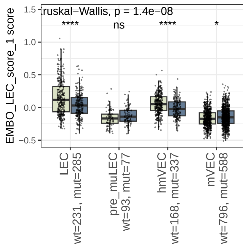
EMBO_LEC_score_1, RAW PVALUE
