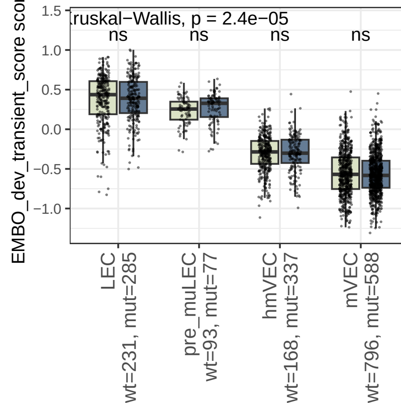
EMBO_dev_transient_score, RAW PVALUE
