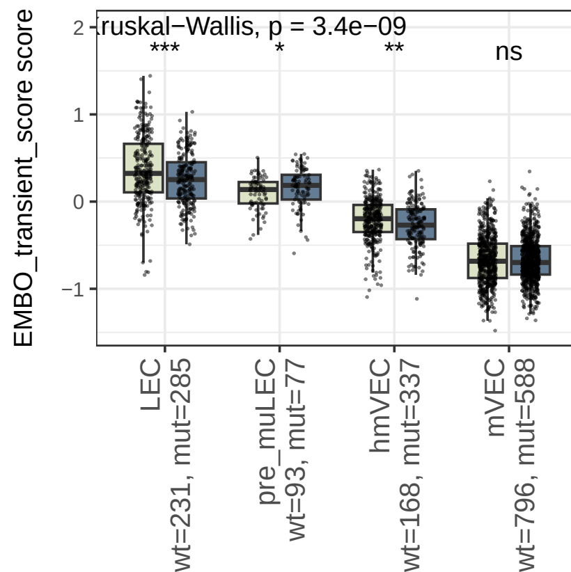
EMBO_transient_score, RAW PVALUE
