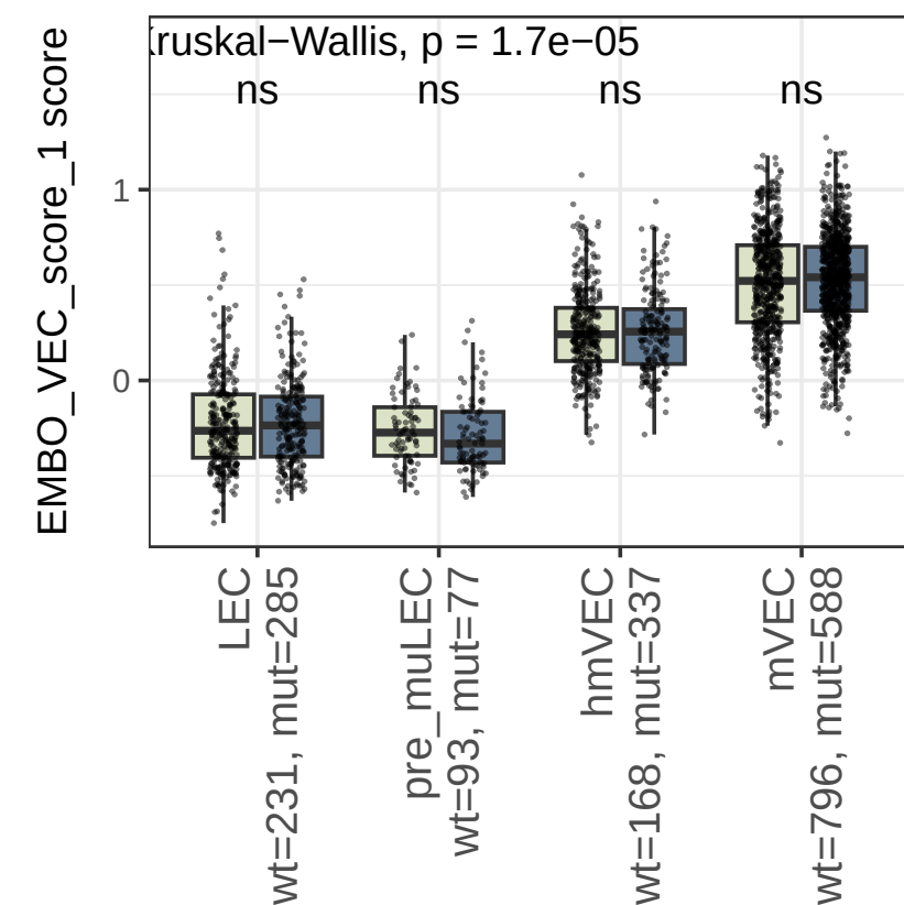
EMBO_VEC_score_1, RAW PVALUE
