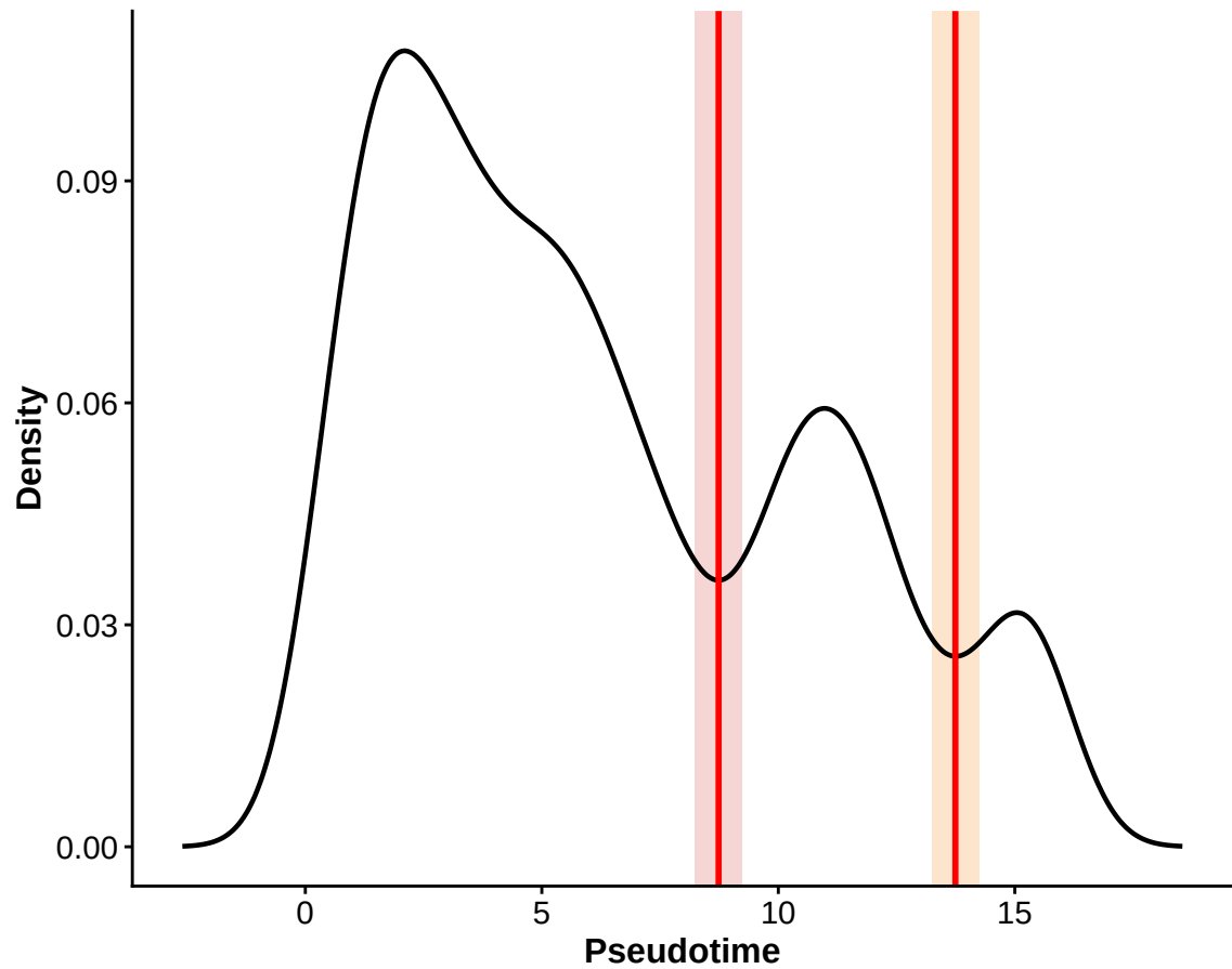
Local Minima Profile (Start: mVEC Lin: 1)
