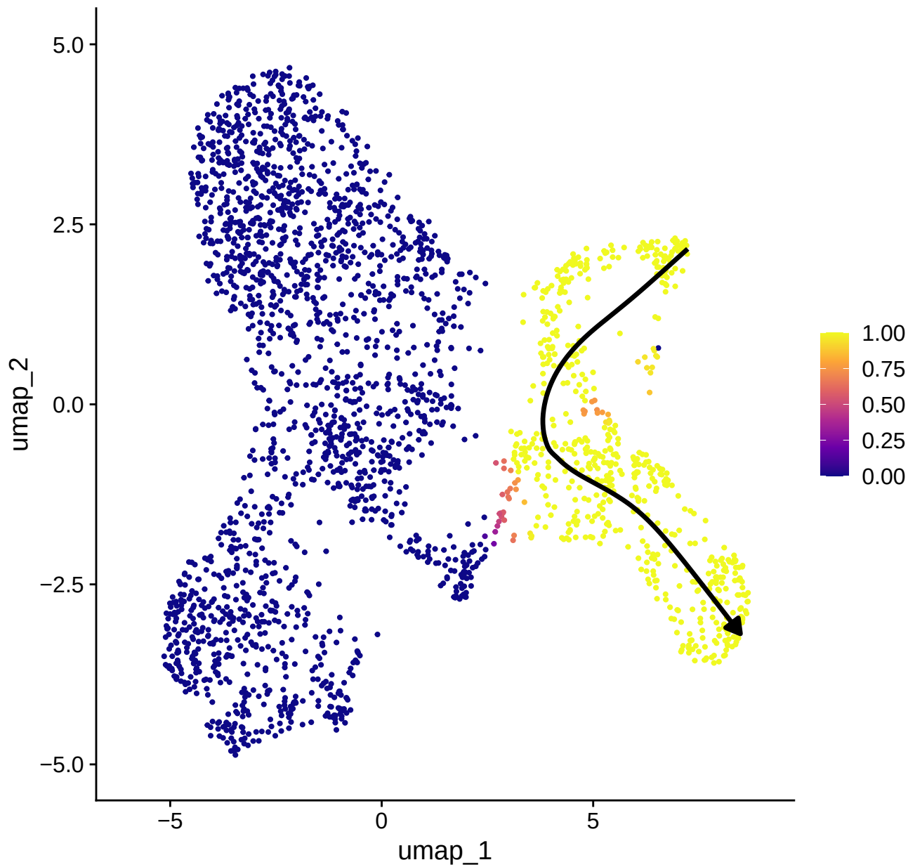
Lineage_Weights_start_LEC_lin2
