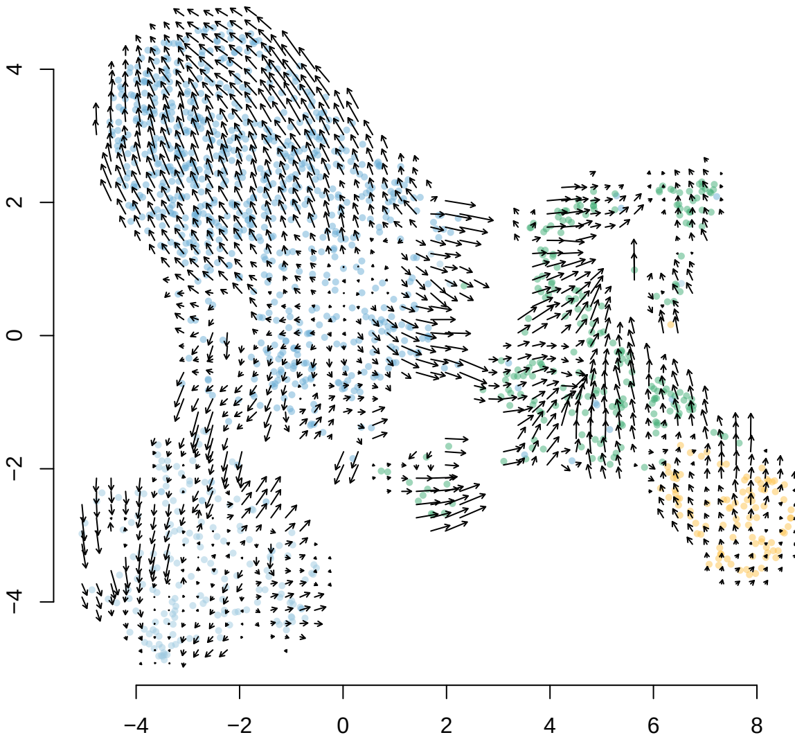
Cell Velocity: S2020_MUT fitquantile=0.02, deltaT=3.0, kCells=10, n=400
