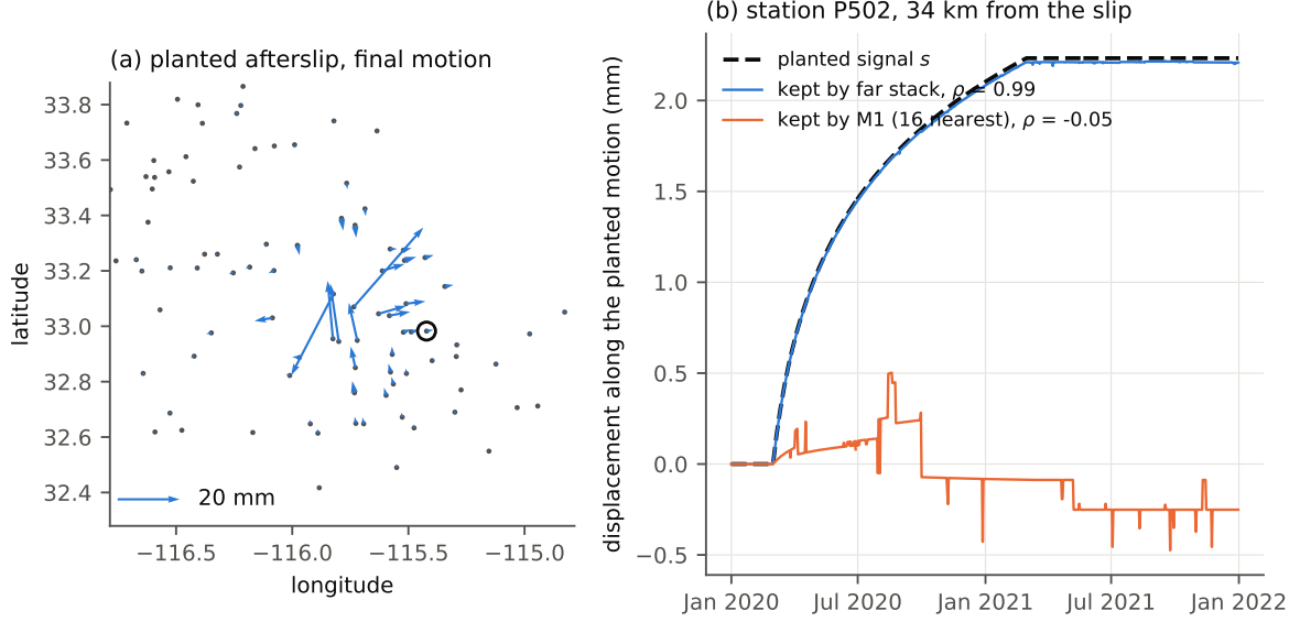
Figure 4: Measuring signal kept. (a) Afterslip planted on a fault of the Community Fault Model: final horizontal displacement at each station, with the slipping patch shaded. (b) At station P502, 34 km from the patch, the planted signal (dashed) and the change it causes in the cleaned series under two filters, projected on the direction of the planted motion; \rho is the retention of Equation (2) at this station. P502 is the station with the median retention under the weighted mean among the 17 stations 15–40 km from the patch. The far stack keeps the signal; the weighted mean of the 16 nearest stations removes it, because its neighbours move with the target.
