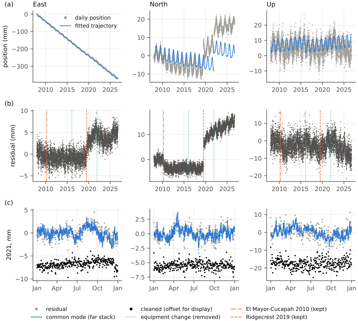
Figure 3: From positions to residuals at station BSRY, about 110 km from the 2019 Ridgecrest earthquakes. (a) Daily positions relative to the first epoch and the trajectory model fitted to 2008–2019; steady plate motion dominates the east component. (b) The residual used by every filter: trend, seasonal terms and equipment steps removed, earthquake offsets kept. (c) One validation year: the residual, the common mode estimated from the rest of the network (the far stack, mean of all other stations) and the cleaned series, shifted down for display. Residuals and common mode are centred on the year’s mean.
