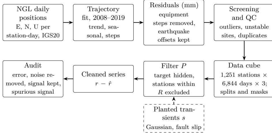
Figure 1: Processing chain from daily GNSS positions to the signal-loss audit. Planted transients are added to the residuals of the data cube, and every filter is run with and without them.
