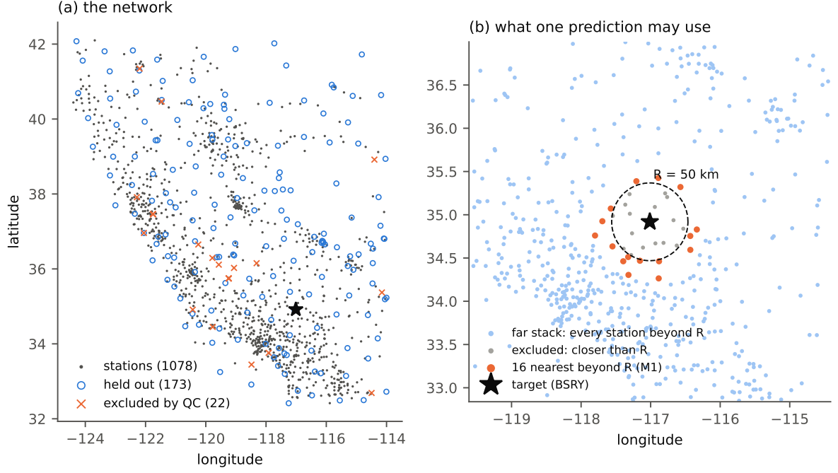
Figure 2: (a) The 1,251 stations used, the 173 held out from all training, and the 22 excluded for non-tectonic site motion. (b) What a prediction for one target station may use at an exclusion radius R = 50 km: stations closer than R are never used; a local filter such as the weighted mean uses the 16 nearest stations beyond R ; the far stack averages every station beyond R .
