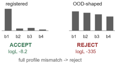
Figure 7. Probability control in chip multi-label learning. (a) val_margin selects the checkpoint with wider positive/negative separation and lower FAR in the development sweep. (b) NB-reject scores the whole 4-bit probability shape rather than only the maximum bit, accepting a registered profile and rejecting an OOD-shaped vector. [Field chip source + domain synthesis]
