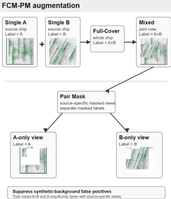
Figure 6. FCM-PM augmentation for chip multi-label learning. Full-Cover CutMix makes an A+B mixed chip, while Pair Mask trains A-only/B-only views to suppress synthetic-background false positives. [Field chip source + domain synthesis]
