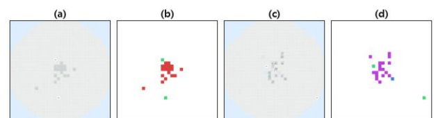
Figure 8. Class separability of raw Failbit Map vs object-id map. Two samples hard to tell apart in raw form ((a), (c)) separate clearly
