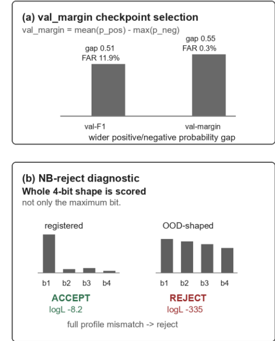
Figure 7. Probability control in chip multi-label learning. (a) val_margin selects the checkpoint with wider positive/negative separation and lower FAR in the development sweep. (b) NB-reject scores the whole 4-bit probability shape rather than only the maximum bit, accepting a registered profile and rejecting an OOD-shaped vector. [Field chip source + domain synthesis]
