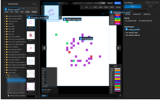
Figure 9. Screenshot of the deployed web application. Search panel, wafer map viewer, chip overlay, measurement panel, navigator thumbnails, and label review are integrated in one screen for large-volume FBM review. [Real operation screenshot]
