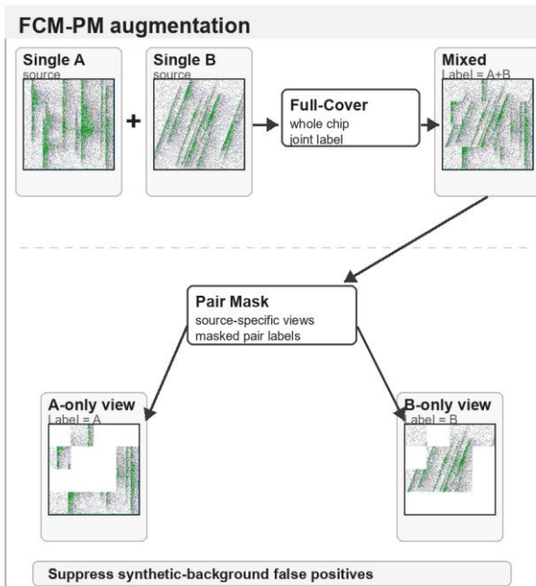
Figure 6. FCM-PM augmentation for chip multi-label learning. Full-Cover CutMix covers the whole chip to make an A+B mixed sample, while Pair Mask makes A-only/B-only views so the synthetic background is not learned as a false positive. [Field chip source + domain synthesis]
