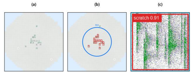
Figure 3. ROI-YOLO 2-stage cascade. Panels show (a) the Failbit Map, (b) the ROI region set by the class prior (blue circle) with YOLO detection boxes inside (red), and (c) the detected chip's scratch detail (confidence 0.91). Failures that look small and scattered globally become distinct under ROI-limited detection and chip-level inspection, while regions outside the ROI are skipped.
