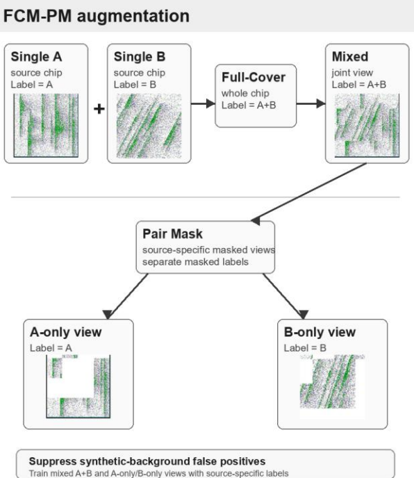
Figure 6. FCM-PM augmentation for chip multi-label learning. Full-Cover CutMix makes an A+B mixed chip, while Pair Mask trains A-
