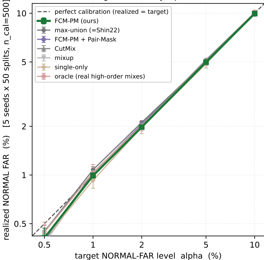
Distribution-free split-conformal calibration: realized FAR tracks target for every operator (max dev 0.15 pp)
