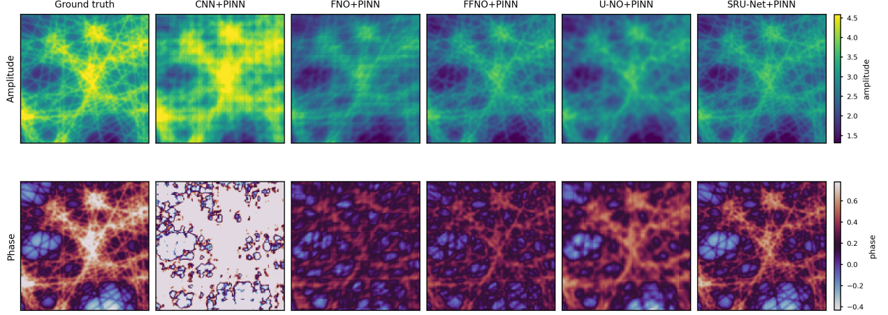
Figure 2: Amplitude and phase reconstruction comparison on synthetically generated CDI data. The cropped comparison shows the target, CNN+PINN, FNO+PINN, FFNO+PINN, U-NO+PINN, and SRU-Net+PINN under the same N = 128 diffraction protocol. Amplitude panels share a target-anchored display scale, and each predicted phase is aligned to the target by a single global circular offset before display. One colorbar is shared across each row.
