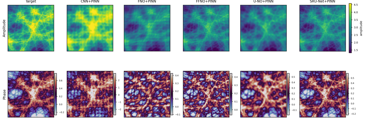
Figure 4: CDI reconstruction comparison with independent phase contrast. This supplemental version of Fig. 2 keeps the amplitude row on the shared target-anchored scale used in the main figure, but scales each phase panel independently using the 1st–99th percentile range after global phase alignment. The phase colors reveal within-panel structure and should not be compared numerically across columns.
