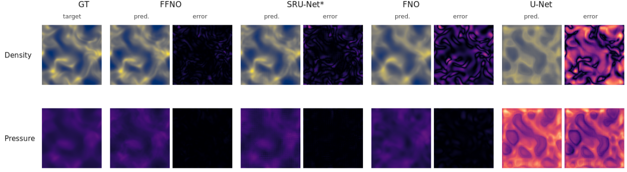
Figure 6: PDEBench CNS fixed-sample predictions and errors. The shared test sample comes from an earlier 2-input-time-step 512/64/64 CNS comparison and shows per-model error structure. Table 6 uses five input states, so this figure should not be read as the visual counterpart of the table.
