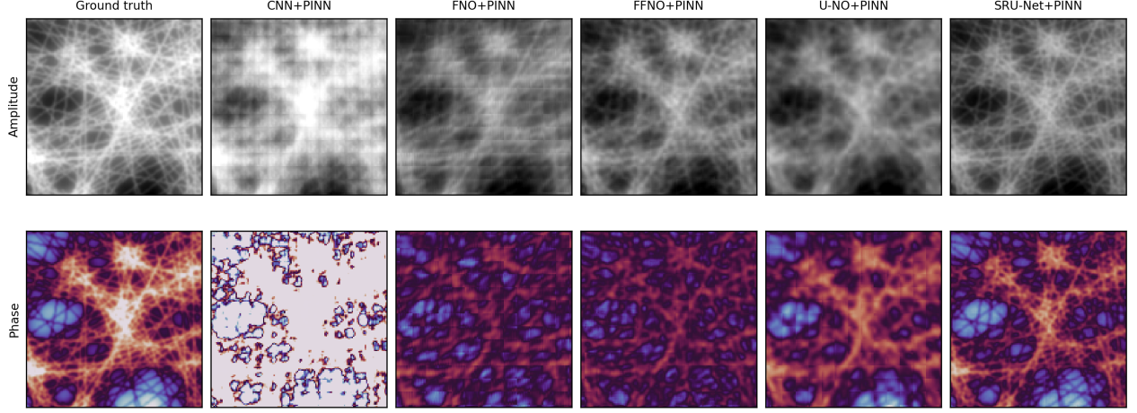
Figure 2: Amplitude and phase reconstruction comparison on synthetically generated CDI data. The cropped comparison shows the target, CNN+PINN, FNO+PINN, FFNO+PINN, U-NO+PINN, and SRU-Net+PINN under the same N = 128 diffraction protocol. Amplitude panels share a target-anchored display scale, and each predicted phase is aligned to the target by a single global circular offset before display.
