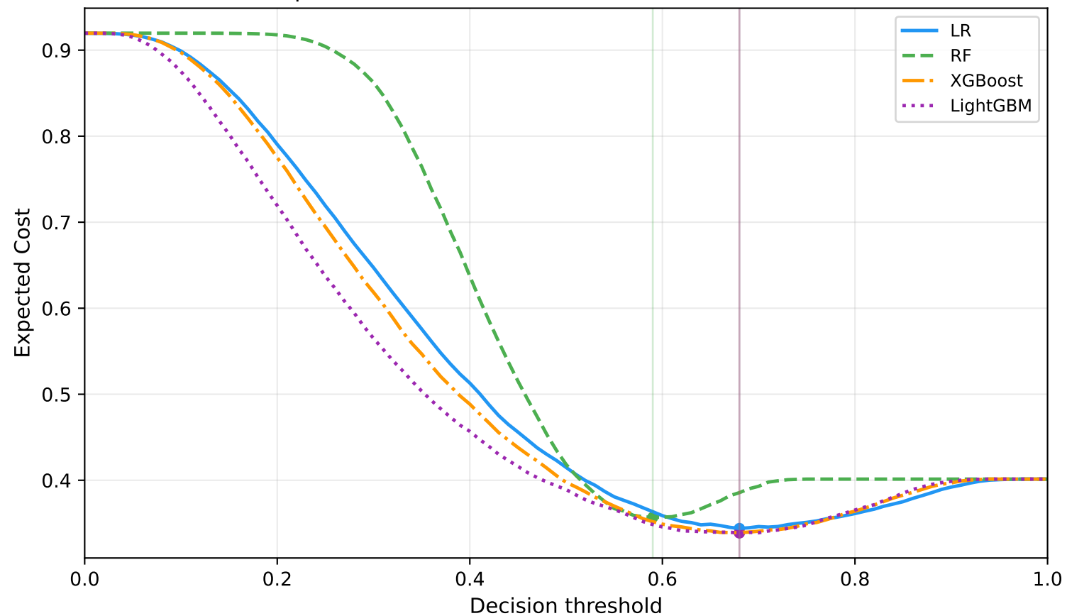
Expected Cost Curves on Home Credit Validation Set
