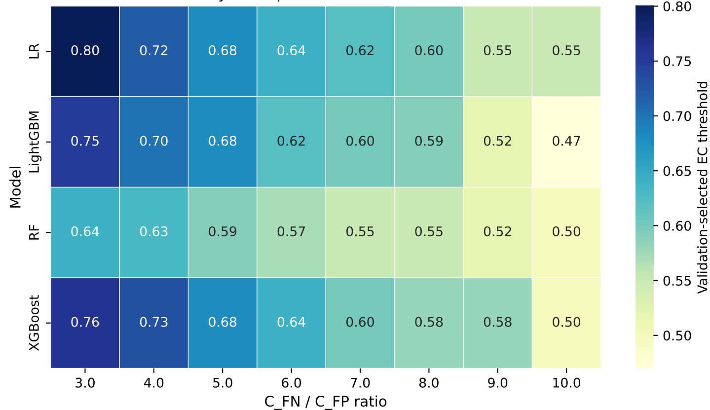
Cost Sensitivity: EC-Optimal Thresholds on Home Credit
