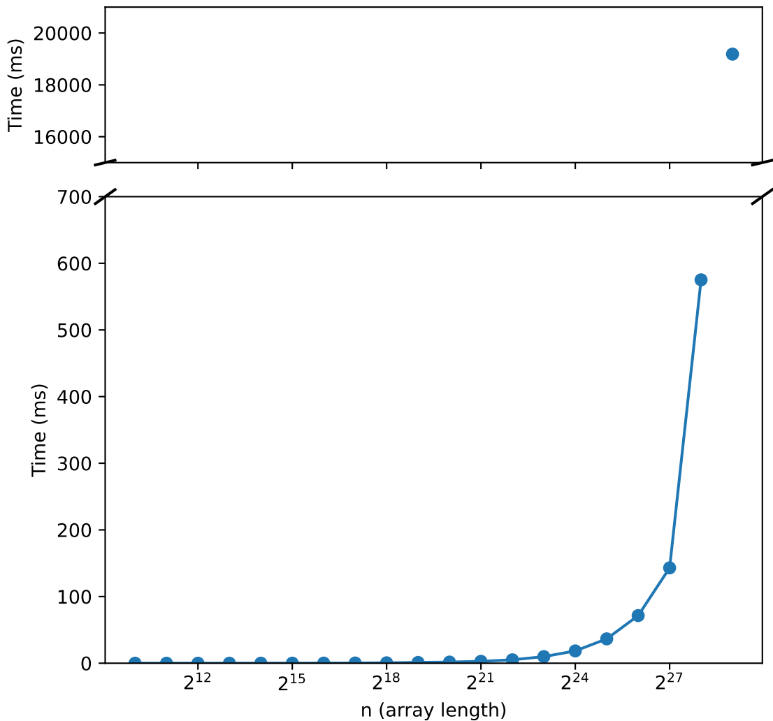
Scaling Analysis of Inclusive Scan (Broken Y-axis)
