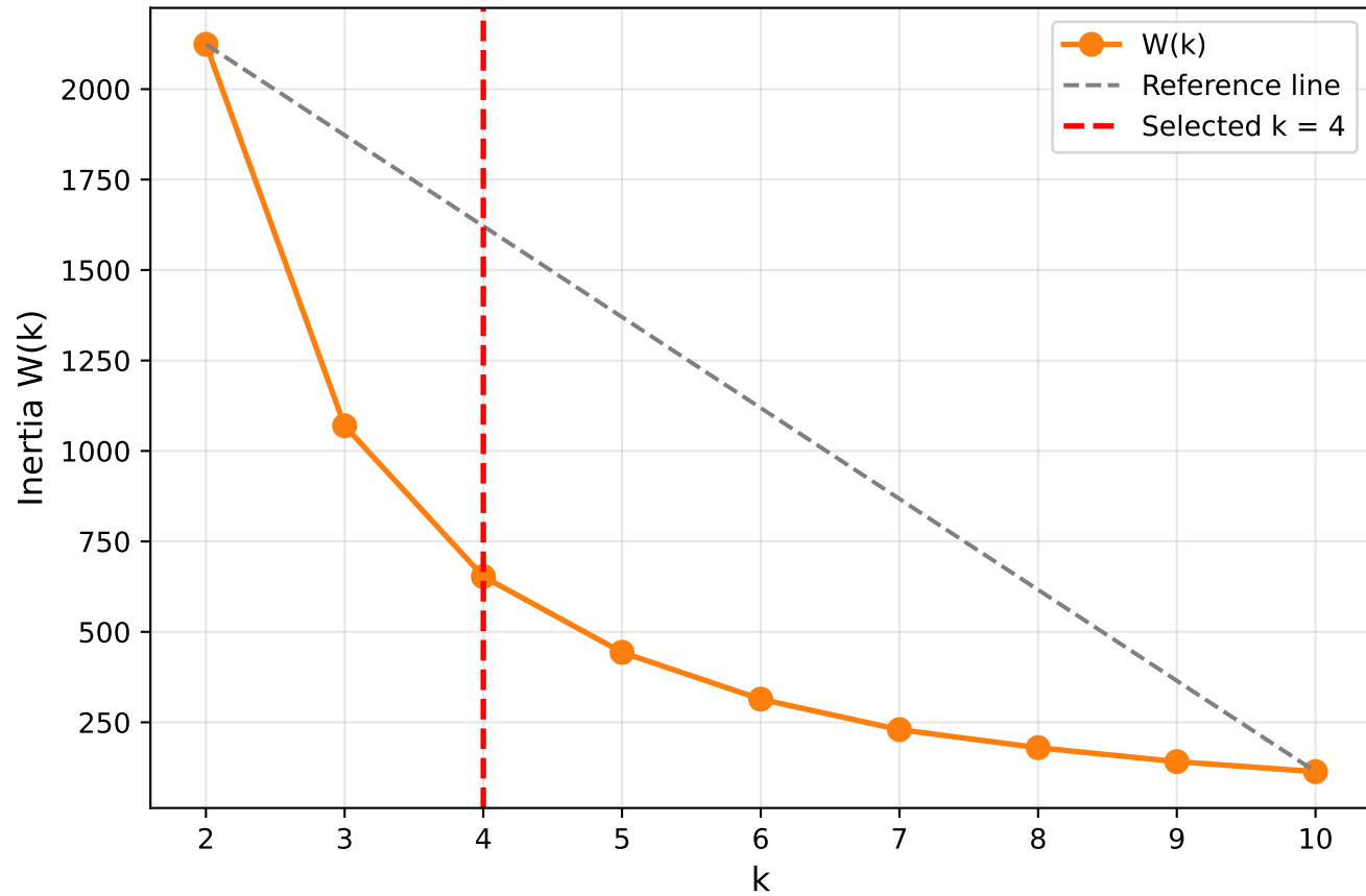
Optimal K for Distance to Hospital Clustering
