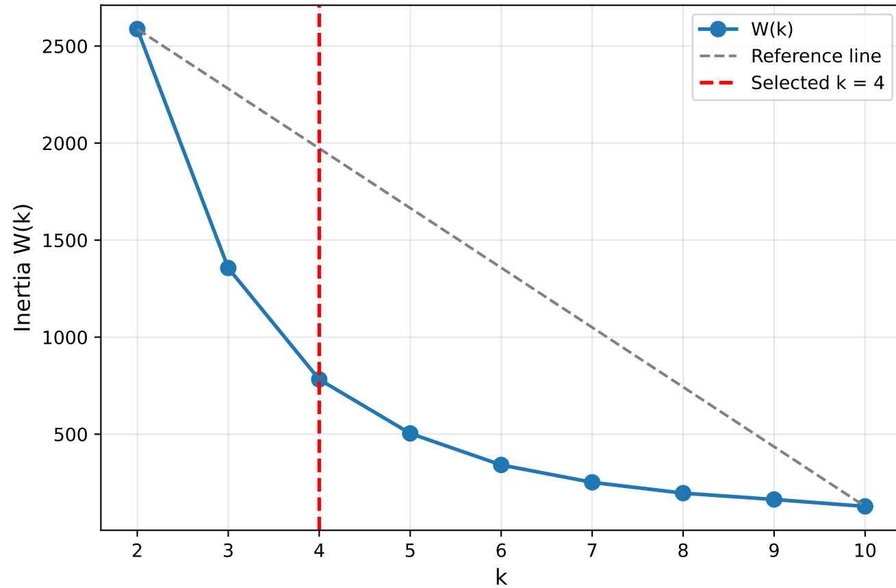
Optimal K for DPFO per Capita Clustering
