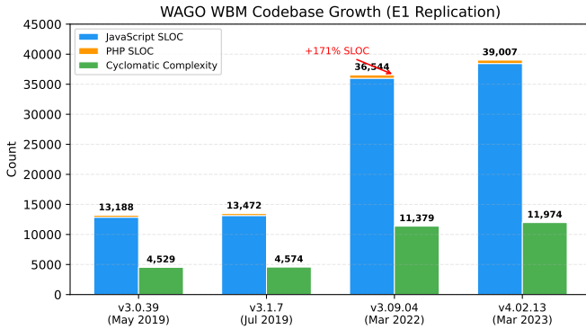
Fig. 1. WAGO WBM codebase growth across four firmware versions, showing total SLOC (stacked JS/PHP) and cyclomatic complexity.
