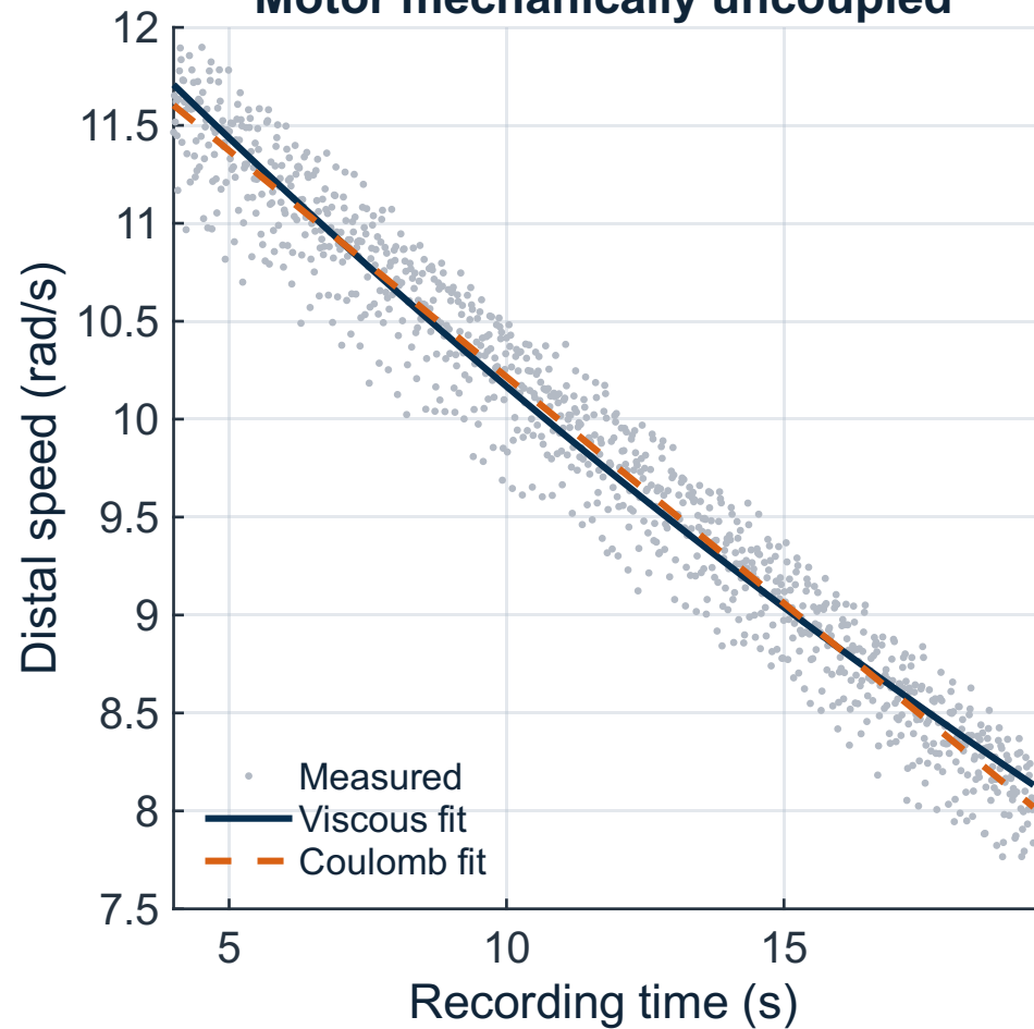
Motor mechanically uncoupled
