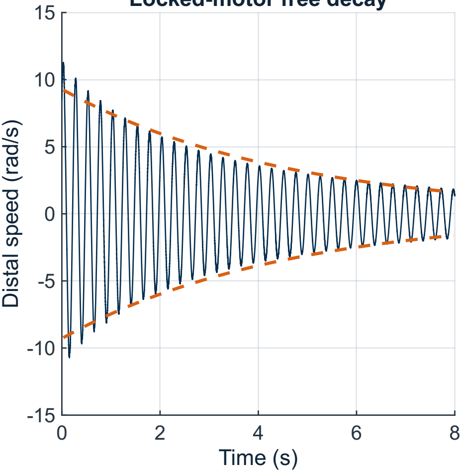
Locked-motor free decay
