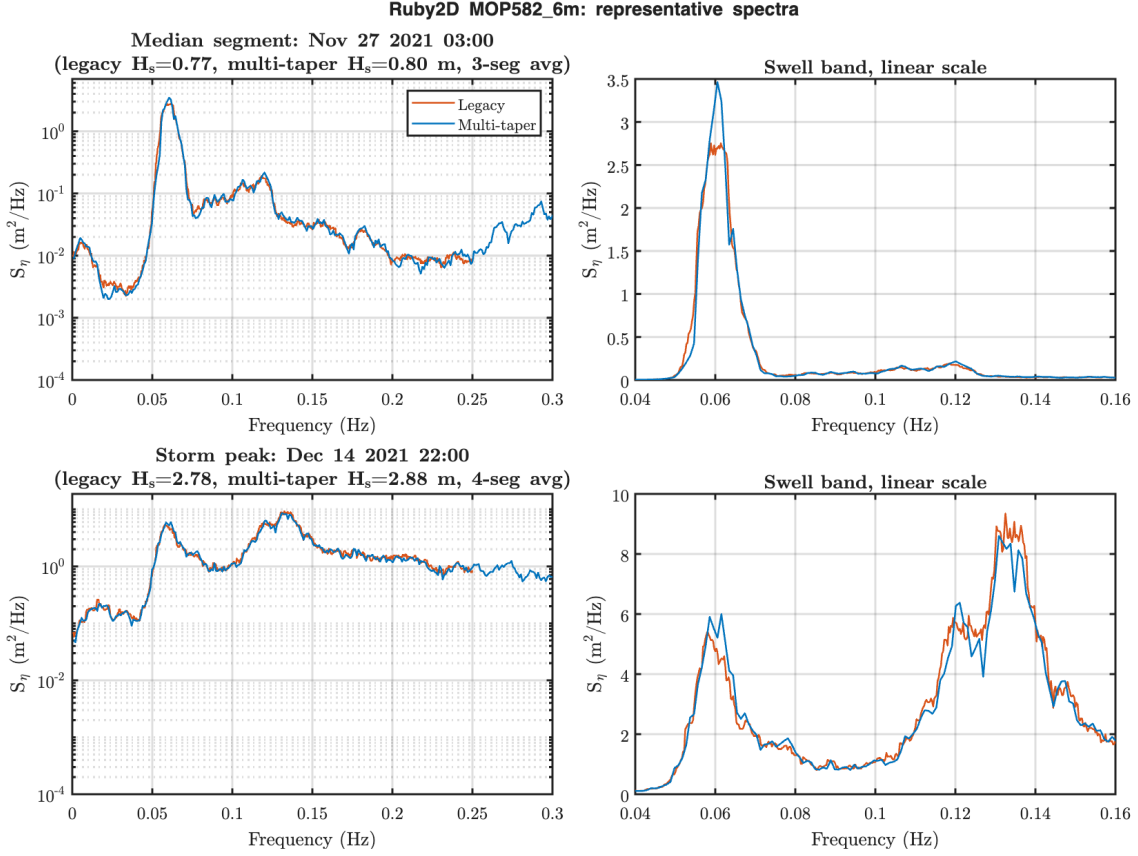
Figure 1: Surface elevation spectra at two representative segments for Ruby2D MOP582_6m. Top: median segment ( H_s = 0.77 m, November 27, 2021). Bottom: storm peak ( H_s = 2.78 m, December 14, 2021). Left: log scale, full SS band. Right: linear scale, swell band detail. The multi-taper estimates (blue) are smoother than the prior single-periodogram estimates (red); peak locations, peak heights, and total variance agree.
