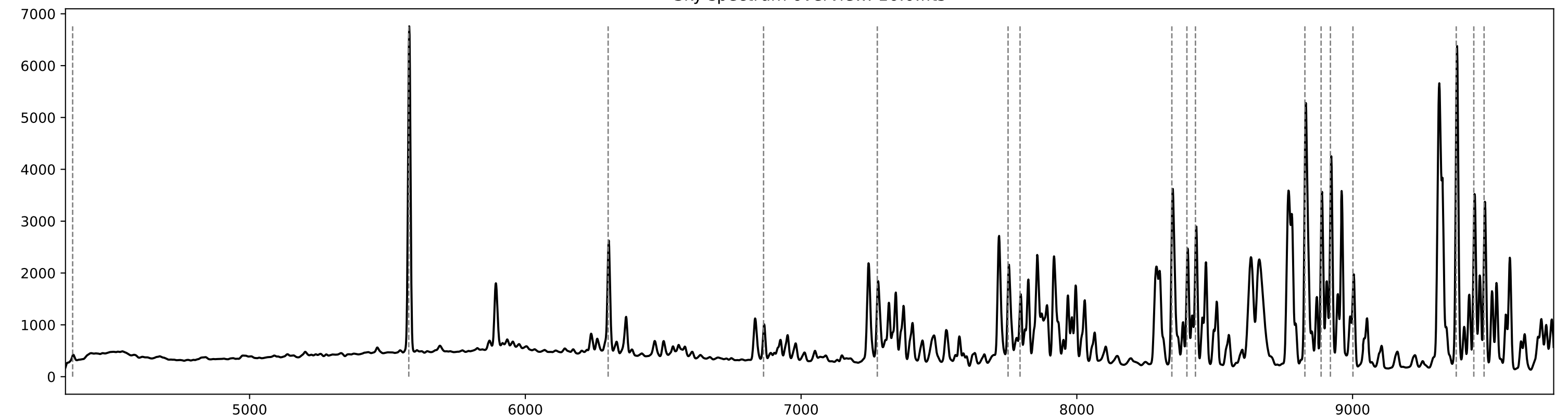
Sky spectrum overview: 16.0.fits
