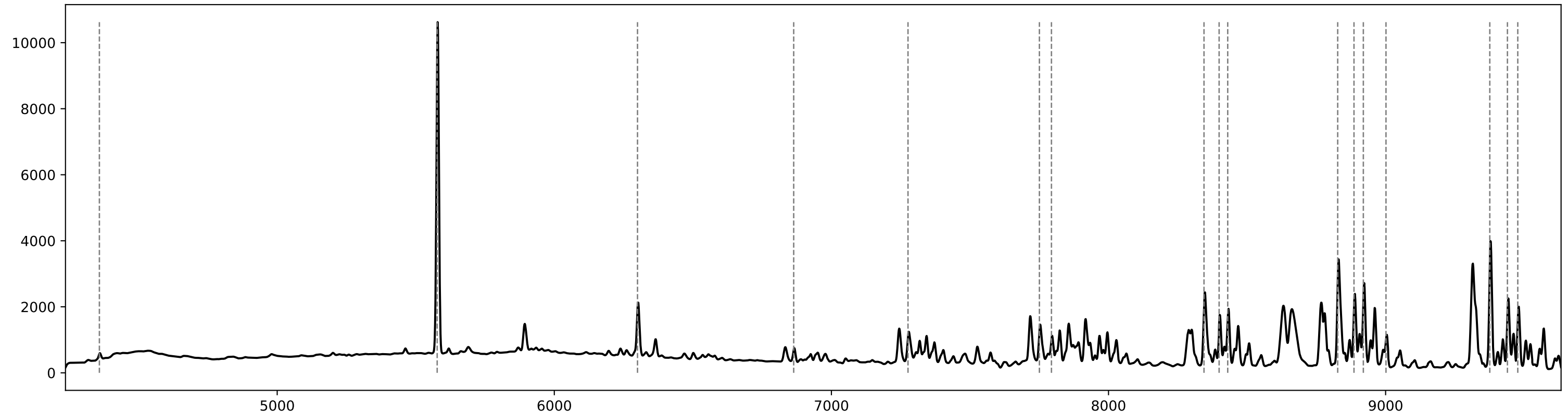
Sky spectrum overview: 23.0.fits
