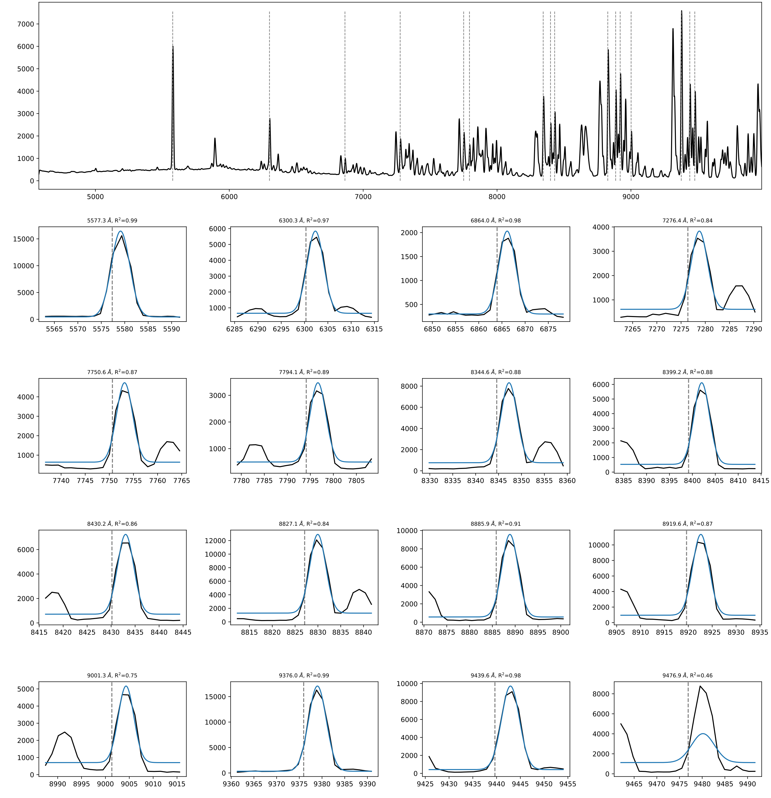
Sky spectrum overview: 119492.fits
