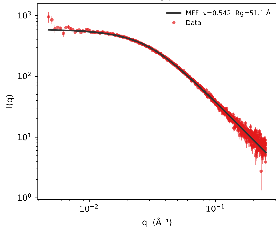
Scattering profile
