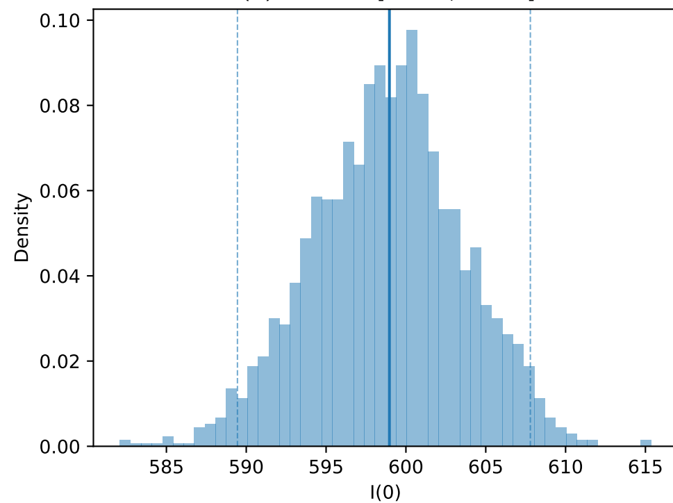
I(0) = 599.0 [589.4, 607.8]
