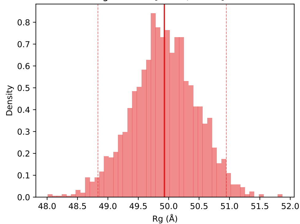
R_g = 49.93 [48.84, 50.95] Å
