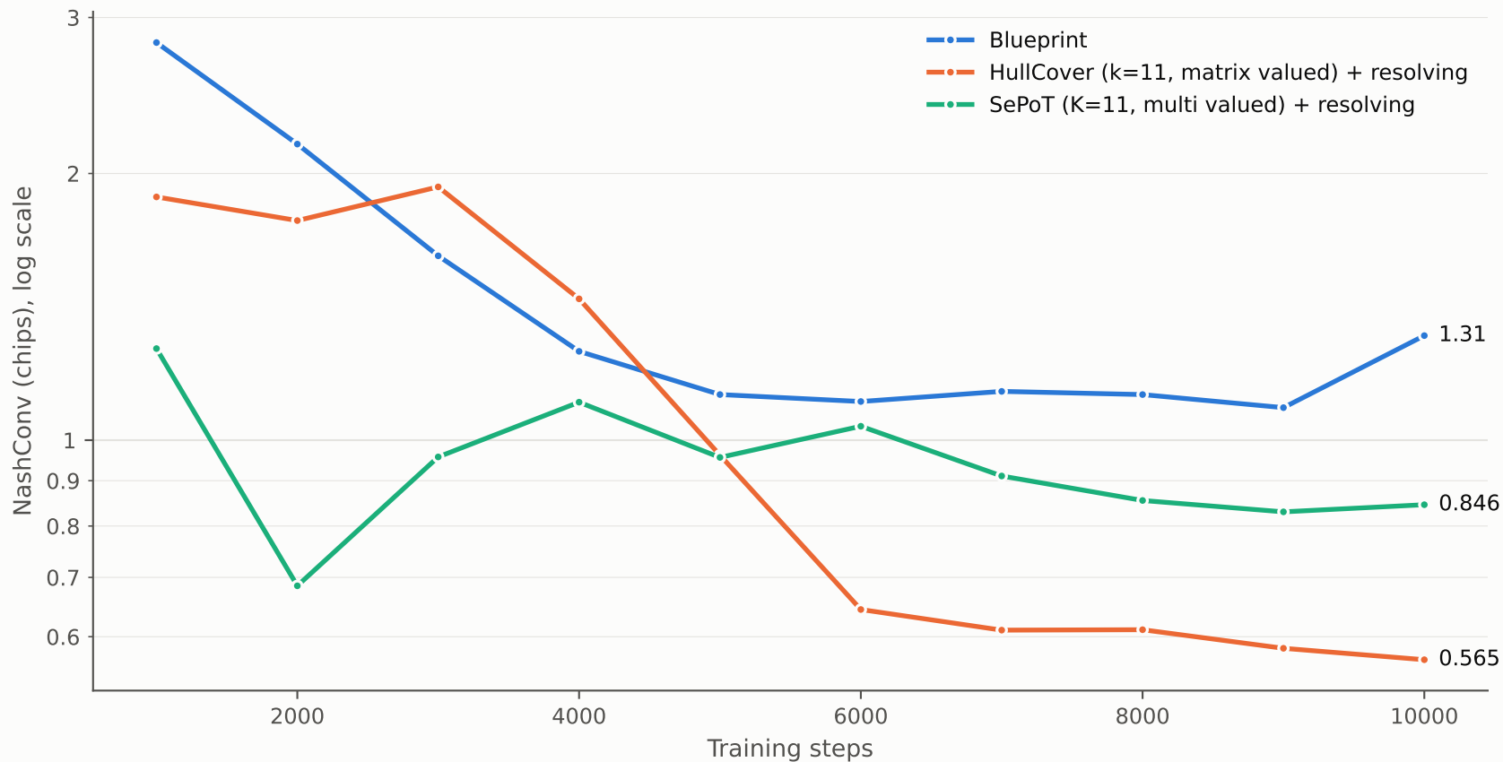
Leduc, paired blueprint: NashConv of the blueprint and with resolving
