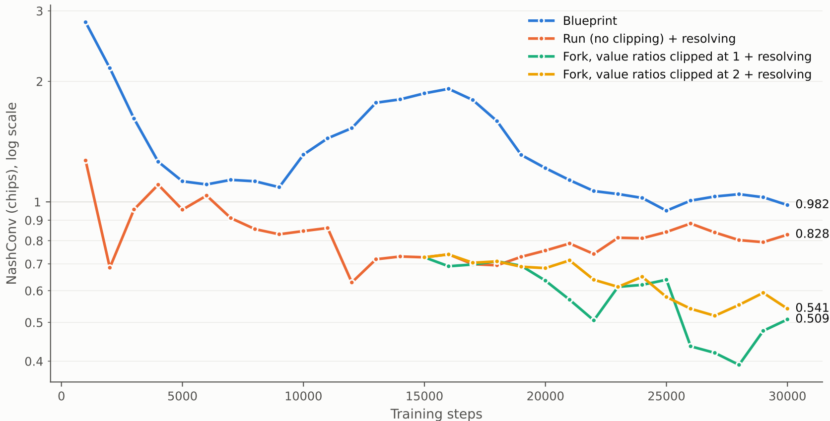
Leduc, multi valued states: resolving with clipped value network ratios (forks at step 15000)
