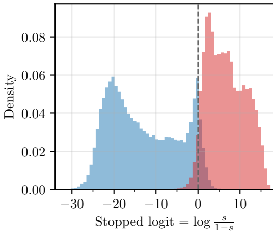
Test logit distribution
