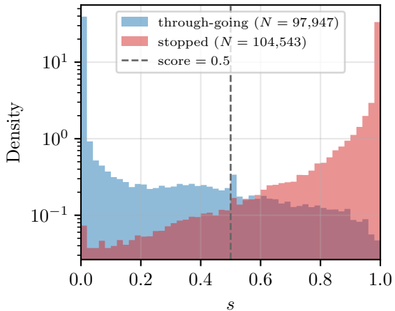
Test score distribution
