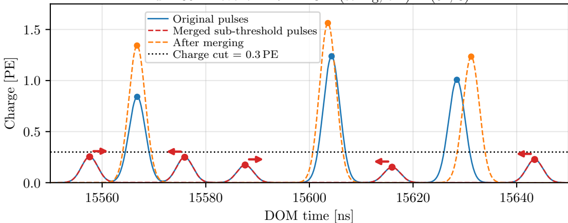
IceCube IC86.2021 burnsample run 136141 event 242722 DOM (string, om) = (61, 3)
