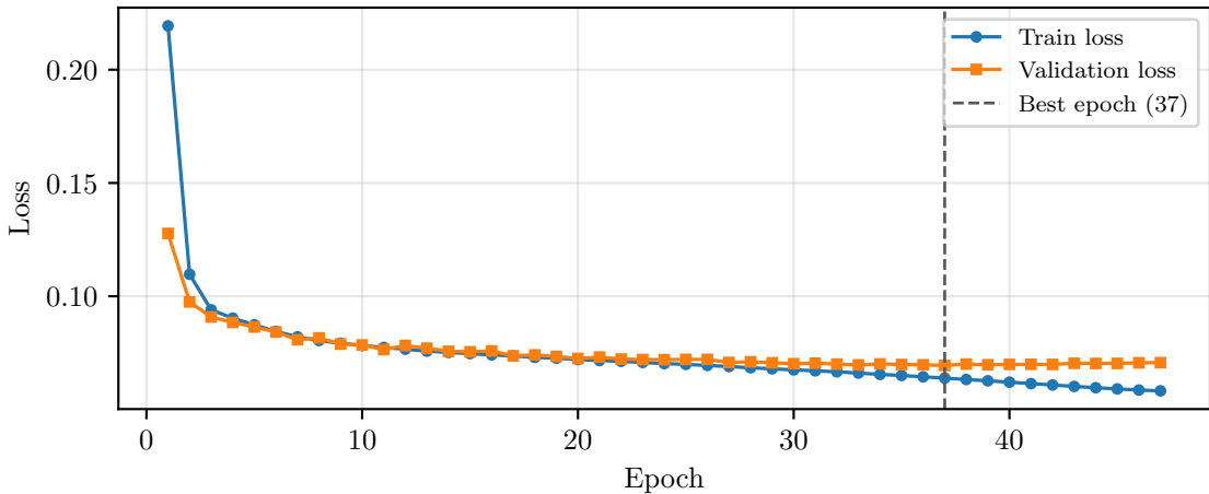
Direction transformer: training history (1,619,920 train / 202,490 val events)
