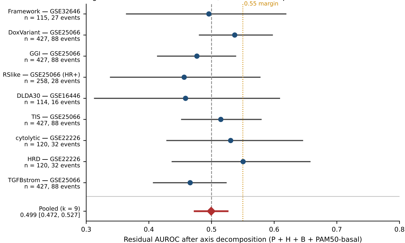
Figure S1. Per-cell residual AUROC, cluster-bootstrap intervals
