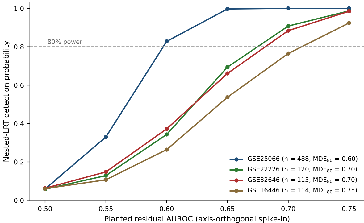
Figure S2. Nested-LRT power against a planted axis-orthogonal signal
