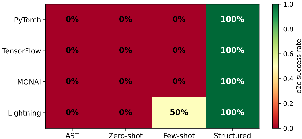
End-to-end FL Runnable Rate by Skill × Framework
