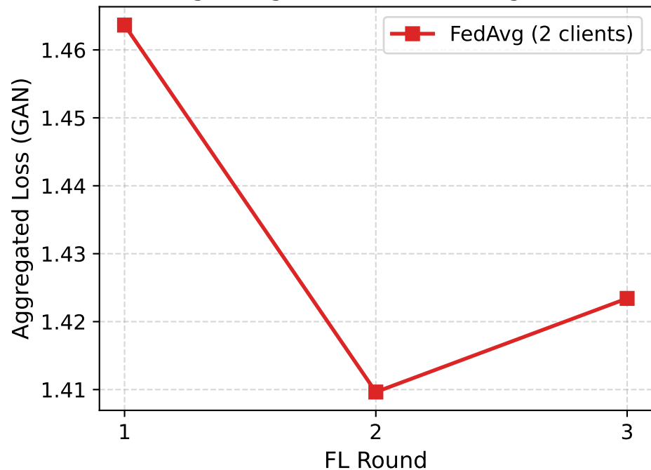
Lightning GAN — FL Convergence
