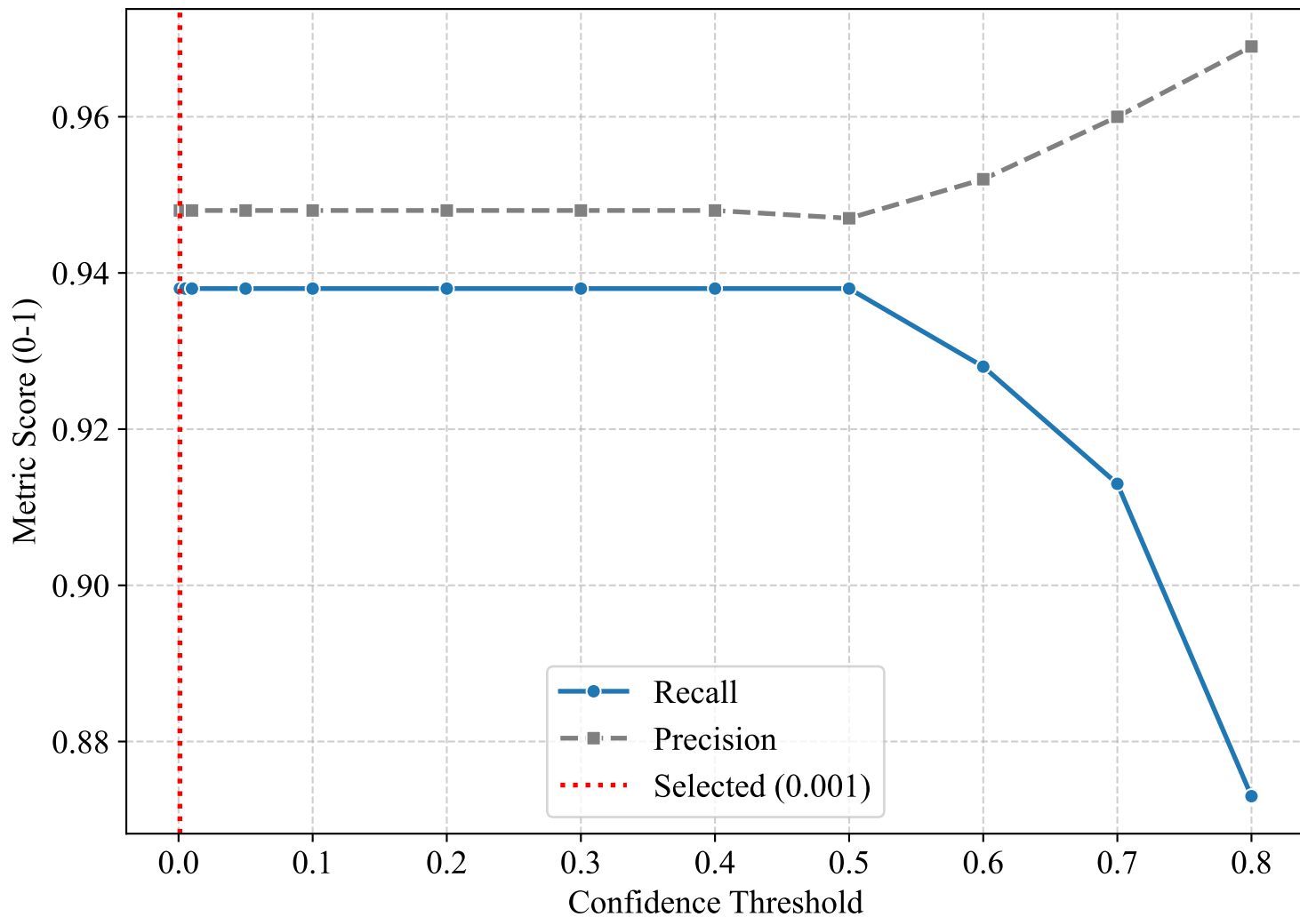
Confidence Threshold Selection: Recall vs. Precision
