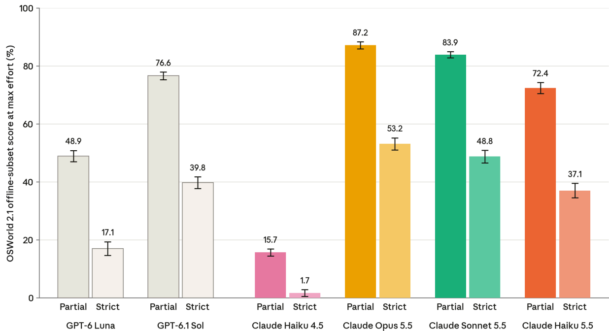
[Figure 8.9.3.A] OSWorld 2.1 (offline subset) scores across models. Bars show the partial score and strict pass rate at max effort (Claude Haiku 4.5: fixed thinking budget), with 95% confidence intervals over the five attempts per task; pale outlined bars are GPT models.
