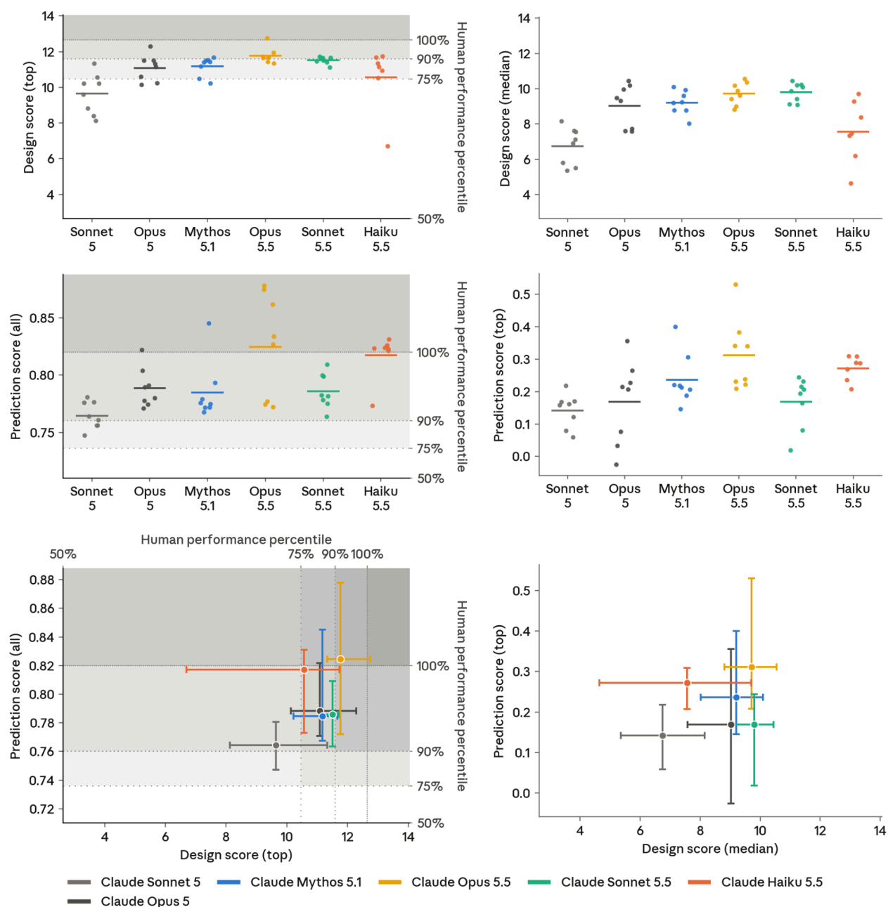
[Figure 2.2.3.1.A] Black-box RNA sequence design. Results of the RNA sequence design task; at least seven attempts per model. Each point is one attempt; the horizontal line is the mean. Throughout the figure, the shaded bands mark human performance percentiles. Top: Design score (top) and design score (median) grade the best and the typical designed sequence. Middle: Prediction score (all) and prediction score (top) are the rank correlation between the model's predicted and measured activity over all sequences and over the top sequences. Bottom: Prediction and design scores plotted against each other. Each crosshair is the full range of data centered on the mean.
