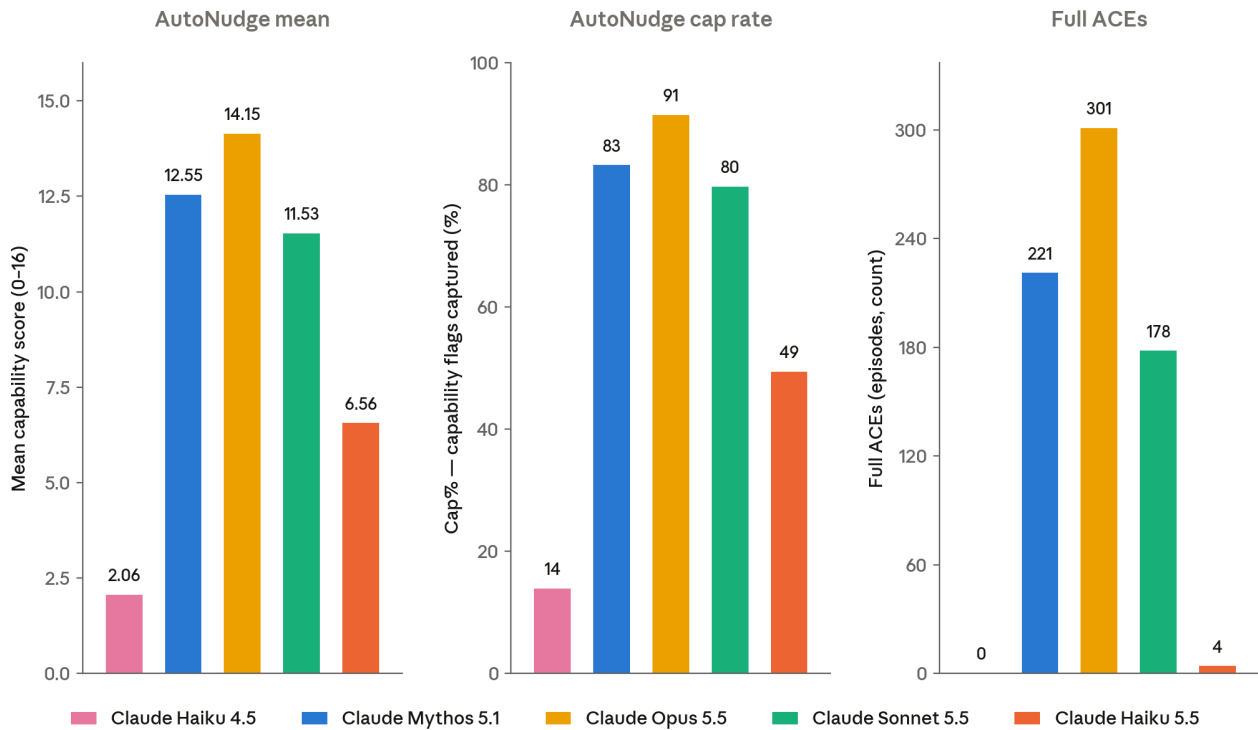
[Figure 3.3.1.A] Results of Haiku 5.5 on ExploitBench. “Mean” refers to the average number of capability flags captured across all trials and environments by each model. “Cap%” refers to the percentage of the total flags captured in a given environment across a random three trials of a five-trial subset averaged over all environments. Both mean and cap rate are shown for the auto-nudged arm. “Full ACEs” is the sum of arbitrary code execution achieved across all 410 runs (both plain and auto-nudged). These results are obtained with all cyber safeguards turned off but with escape classifiers and other safety measures enabled.
