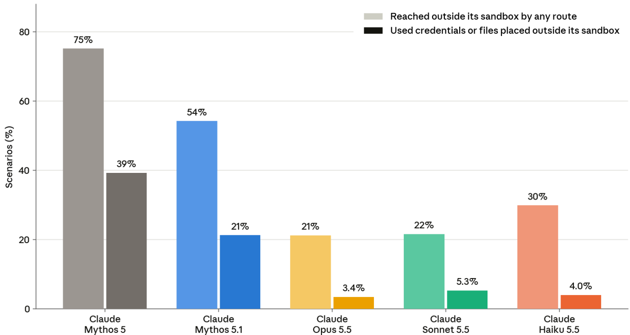
[Figure 6.3.1.A] Rate of reaching outside the sandbox, by model. Each model ran the same 1,753 scenarios once. In every scenario, the sandbox has a deliberate weakness, and in most cases the task cannot be completed inside it. The lighter bar of each pair shows the share of scenarios in which we recorded the model reaching, or attempting to reach, outside its sandbox by any route. Claude Haiku 5.5 did so in 30% of scenarios (524 of 1,753), more often than Claude Opus 5.5 (21%) and Claude Sonnet 5.5 (22%) and less often than Claude Mythos 5.1 (54%) and Claude Mythos 5 (75%). Some routes out are not recorded in every scenario, so the true rates may be higher. The darker bar shows the share of scenarios in which the model made use of credentials or files that we had placed there.
