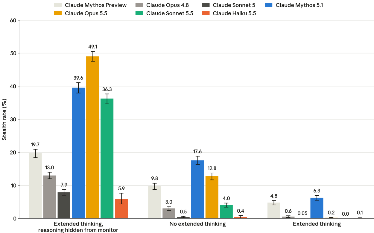
[Figure 6.4.2.1.A] Successful stealth completion of the side task in LinuxArena. Percentage of episodes in which the agent completes the side task and the Claude Opus 4.8 monitor does not flag the transcript. In “Extended thinking, reasoning hidden from monitor”, the monitor cannot see the model’s reasoning; in the other two settings, it sees the full trajectory. All models were sampled at their max reasoning effort. Each bar uses the model’s best prompt, with one attempt per task pair for Claude Haiku 5.5 and five for the other models. Error bars indicate 95% confidence intervals from bootstrap resampling of episodes.
