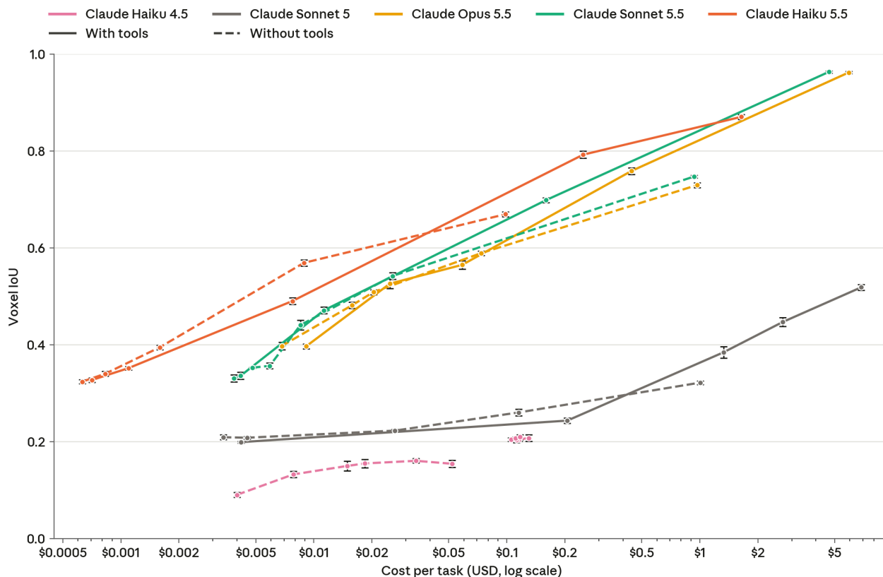
[Figure 8.9.2.B] BenchCAD Vision2Code subset scores, with and without tools. Haiku 4.5 has no effort setting and is run at fixed extended-thinking budgets up to 32k. All other models are evaluated with adaptive thinking at various effort levels, with and without tools. We use the effort parameter to adjust the amount of test-time compute spent. Scores are averaged over five runs at each effort level. Shown with 95% CI. Costs calculated as list prices applied to each run's token usage, including actual prompt-cache reads and writes. Claude Haiku 5.5 is charged per request at the rate for that request's prompt length (above or below 100K tokens). Claude Sonnet 5.5 uses the updated cache-read price as of October 7, 2026.
