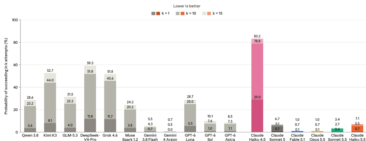
[Figure 5.2.1.A] Indirect prompt injection attacks from the Gray Swan IPI benchmark (Q1+Q2 2026) , lower scores are better. All models use extended thinking. Results represent the probability that an attacker finds a successful attack after k=1 , k=10 , and k=15 attempts. Qwen 3.8, DeepSeek-V4-Pro, and GLM-5.3 were not evaluated on GUI Computer use scenarios. Claude models are evaluated without protections specific to prompt injection.
