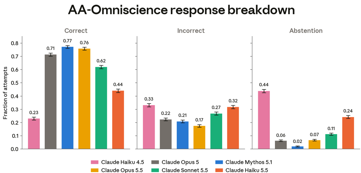
[Figure 6.3.3.1.B] AA-Omniscience breakdown. Grade breakdown on the AA-Omniscience closed-book factuality benchmark. Each response was graded as correct, incorrect, or an abstention.
