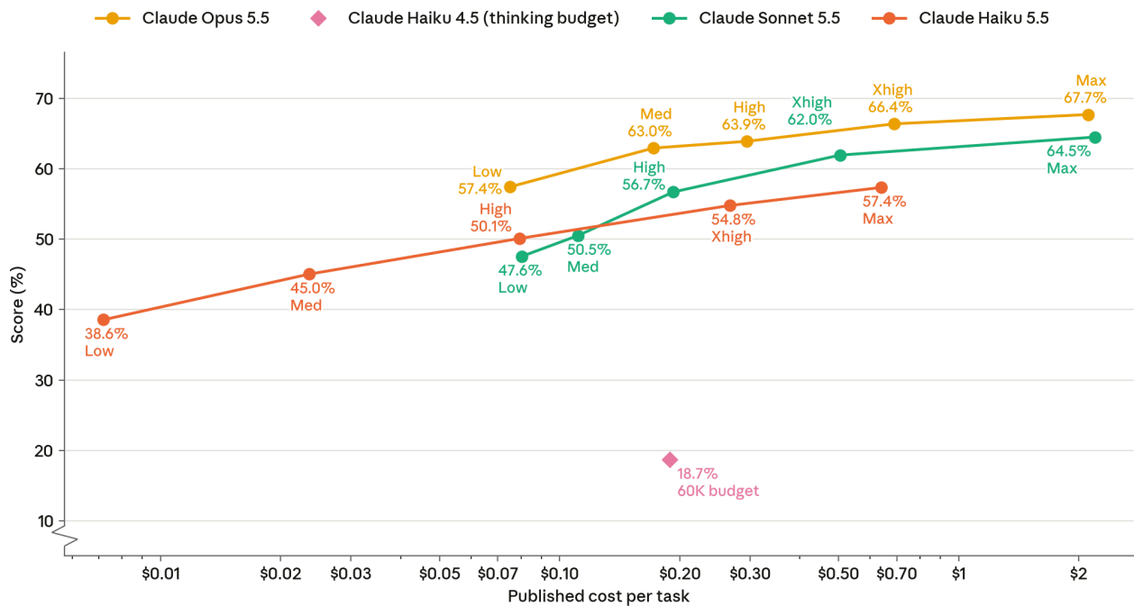
[Figure 8.8.1.A] Humanity's Last Exam (HLE, with tools) reasoning effort scaling. Accuracy on HLE as reasoning effort scales from low to max against average cost per task (log scale). Costs for Opus 5.5 and Sonnet 5.5 assume a perfect cache hit rate; Haiku 4.5 and 5.5 use list prices on recorded usage, with web search fees excluded. Claude Haiku 4.5 is shown at a 60K-token extended-thinking budget with 160K task budget.
