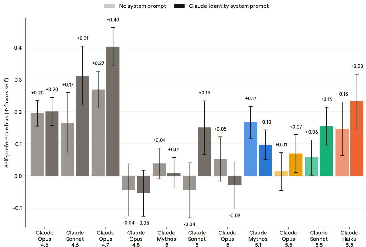
[Figure 6.3.2.A] Self-preference bias by model and prompting condition. Positive values indicate more lenient scores when the grader is told the transcript author is Claude. This is shown on a 0–9 scale, so the values here are much smaller than the maximum possible. Shown with paired 95% CIs. Without a system prompt, 127 of Haiku 5.5’s 2,000 ratings (about 6%) could not be scored, and the missing ones were unevenly spread across the stated authors.
