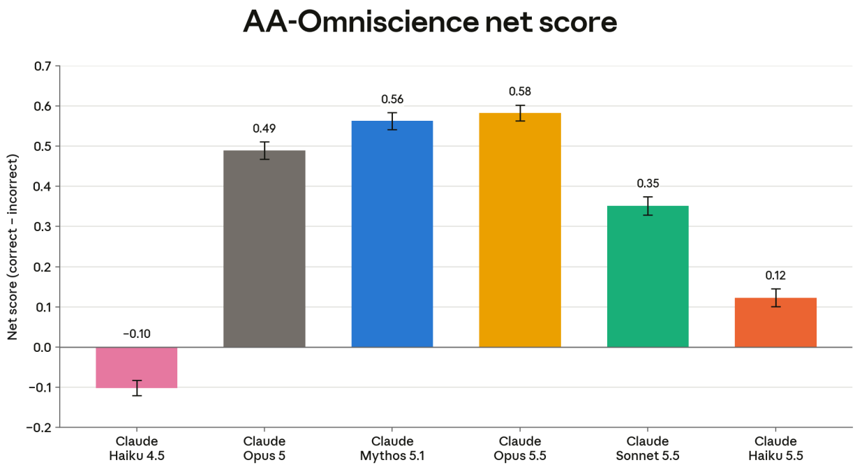
[Figure 6.3.3.1.A] AA-Omniscience net scores. Net score is the fraction of correct responses minus the fraction of incorrect responses on AA-Omniscience.
