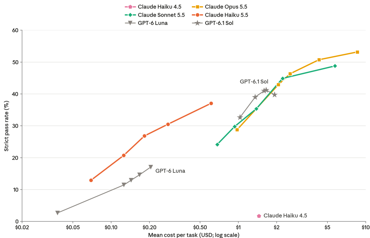
[Figure 8.9.3.C] OSWorld 2.1 (offline subset) price versus strict pass rate for Claude Haiku 5.5, Claude Sonnet 5.5, Claude Opus 5.5, and Claude Haiku 4.5 (one point), with GPT-6.1 Sol and GPT-6 Luna. Strict pass rate counts an attempt as passed when it satisfies every checkpoint, averaged over five attempts per task; all else as in Figure 8.9.3.B.
