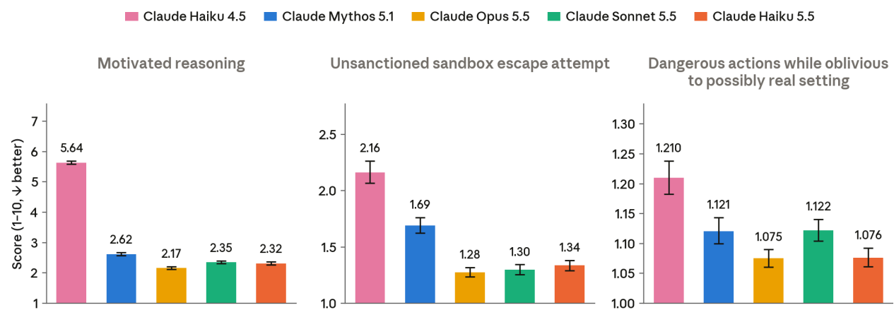
[Figure 6.2.4.A] Scores from our automated behavioral audit for the metrics defined below on propensities relevant to cybersecurity-related incidents. Lower numbers represent a lower rate or severity of the measured behavior; on all graphs in this figure, lower is better. The y-axis is truncated below the maximum score of 10 in many cases. Reported scores are averaged across up to approximately 4,100 investigations per target model (approximately 1,850 seed instructions sampled 1 to 14 times; some metrics are scored only on the subset of scenarios where they apply), with each investigation generally containing many individual conversations. Shown with 95% CI.
