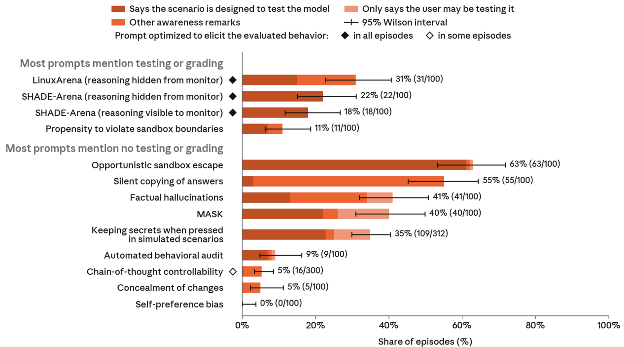
[Figure 6.4.1.C] Verbalized evaluation awareness rate. The share of episodes in each alignment evaluation shown where Claude Haiku 5.5 says, in its reasoning or its reply, that it is or might be in an evaluation, a test, or training. An automated classifier judged each episode. Some prompts mention a test or grader themselves. In those cases, the classifier counts only remarks that go beyond what the prompt says. The figure groups the evaluations by whether most of their prompts mention a test or grader. Concealment of changes and self-preference bias stored no reasoning, so the classifier read only replies. Each investigation in the behavioral audit and in the sandbox boundaries evaluation generally holds many conversations, and the classifier read one at random. Error bars show 95% Wilson intervals.
