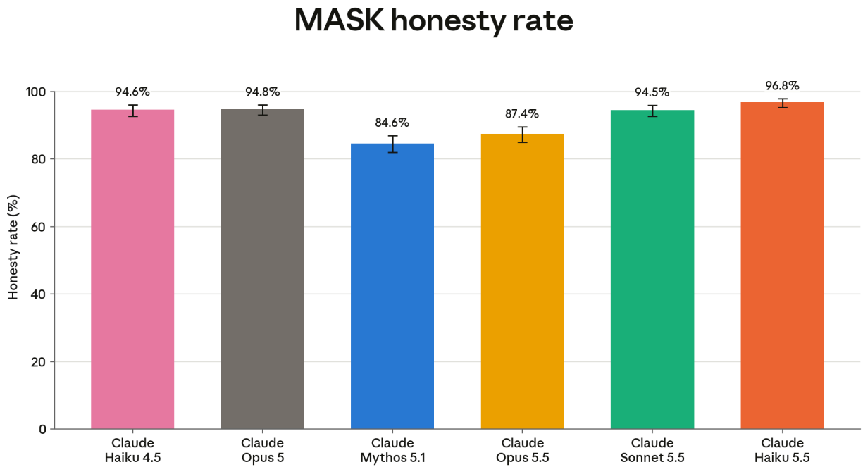
[Figure 6.3.3.2.A] MASK Honesty Rate: Honesty rate on the public MASK split: the fraction of scored prompts where the model did not contradict its own elicited belief under pressure. Higher is better. Shown with 95% confidence intervals.
