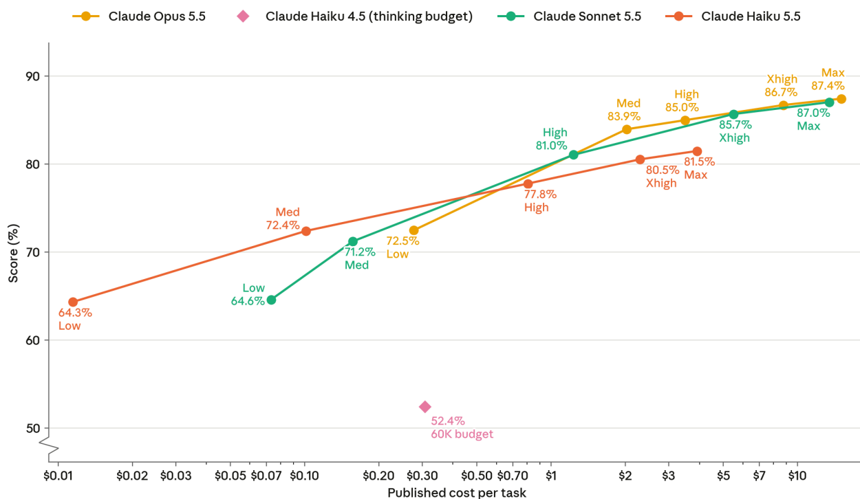
[Figure 8.8.2.A] DRACO score versus average cost per task across reasoning effort levels. Normalized score on DRACO at a 980k task budget as reasoning effort rises from low to max against average cost per task (log scale). Costs for Opus 5.5 and Sonnet 5.5 assume a perfect cache hit rate; Haiku 4.5 and 5.5 use list prices on recorded
