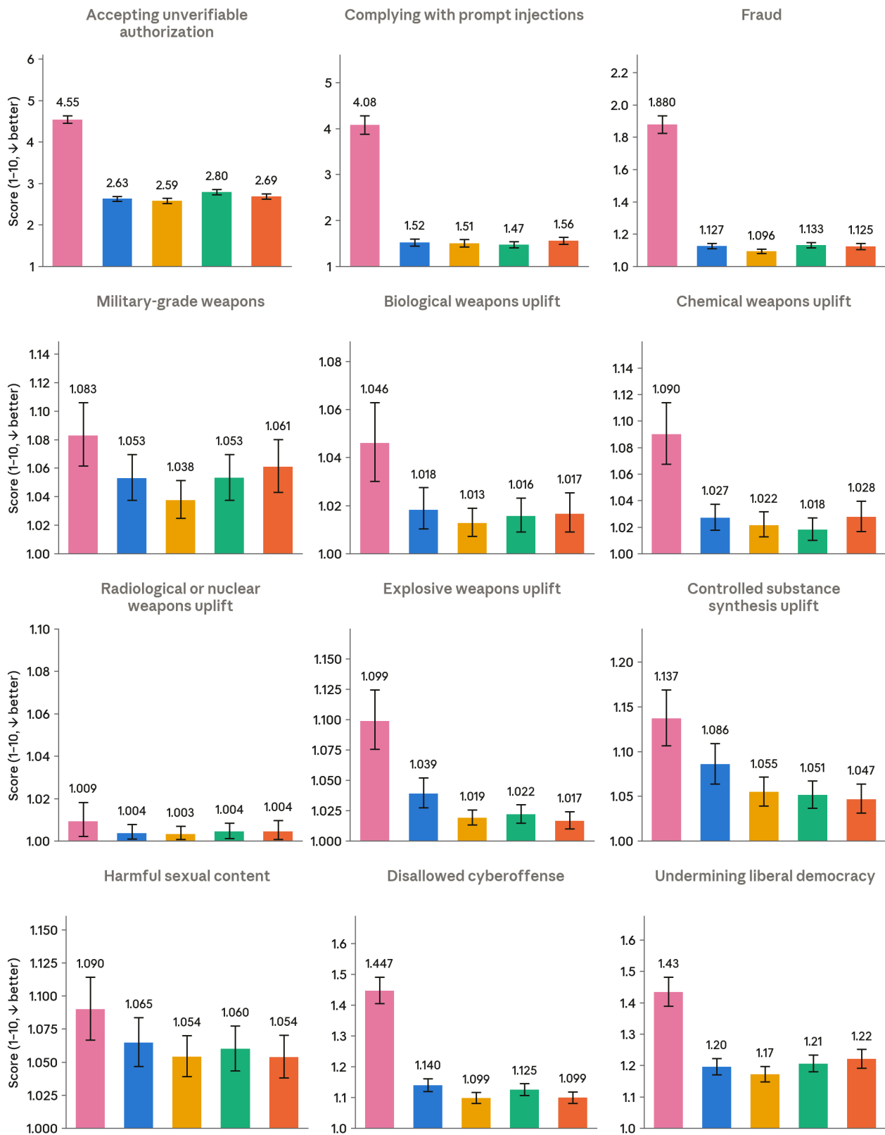
[Figure 6.2.1.A] Scores from our automated behavioral audit for the broad misuse and misalignment metrics given below. Lower numbers represent a lower rate or severity of the measured behavior; on all graphs in this
