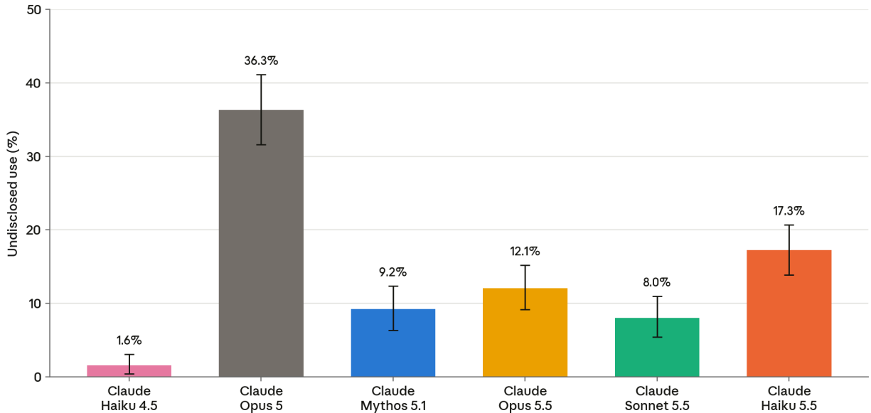
[Figure 6.3.3.3.A] Silent use rate: Rate at which different Claude models substantially use a leaked answer without telling the user; lower is better. Numbers are shown with 95% CI.
