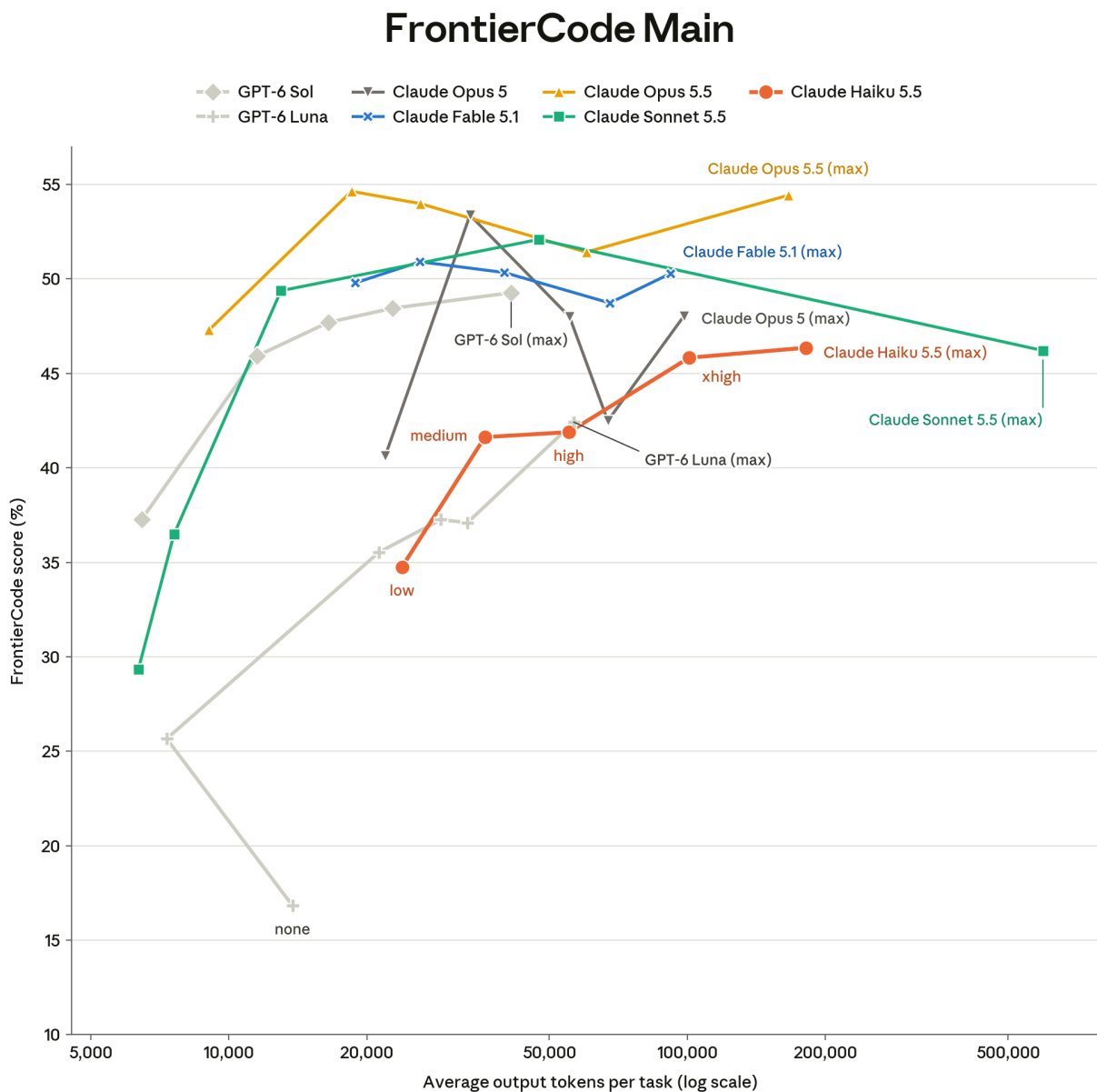
[Figure 8.3.A] FrontierCode Main score versus average output tokens per task across reasoning effort levels ( low , medium , high , xhigh , and max ; GPT-6 Luna also at none ). Cognition ran the evaluation for every model shown and reported the results; Claude models were run in Claude Code, and GPT models were run in Codex. Cognition's result files report token counts for every model and no cost for Claude Haiku 5.5, so the x-axis shows average output tokens per task, on a logarithmic scale. Each Claude Haiku 5.5 point is labeled with its effort level (its max point with the model's name). Every other model is labeled with its name at its max point, and GPT-6 Luna's none point is also labeled with its effort level. Each line joins a model's points in order of
