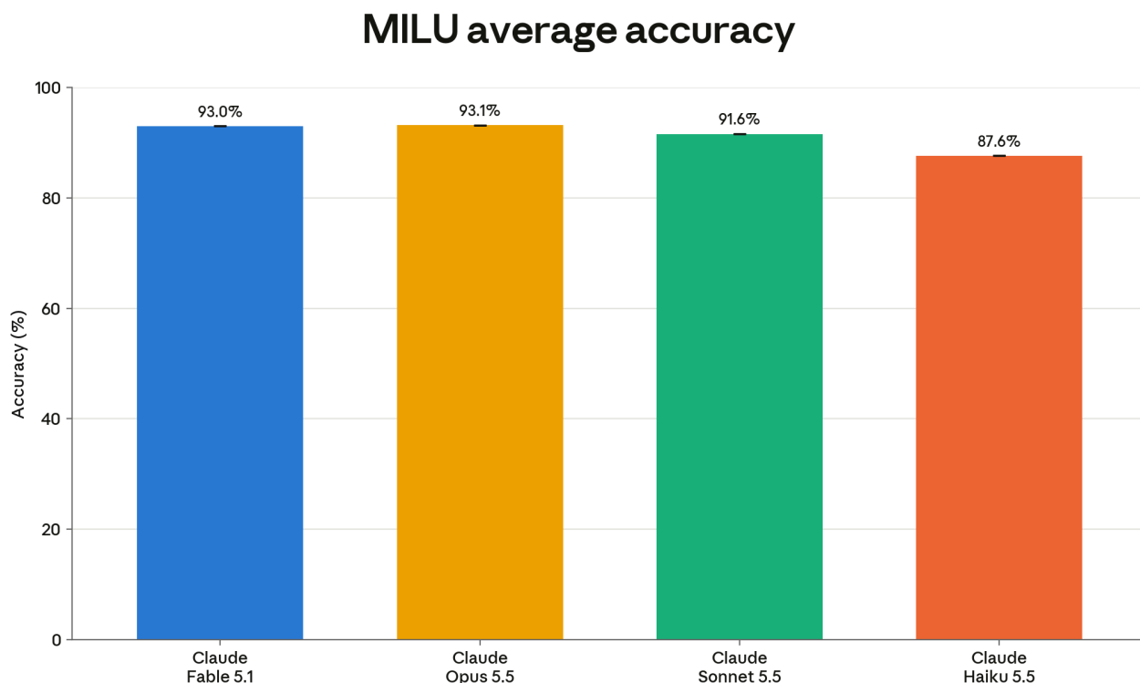
[Figure 8.12.2.A] MILU average accuracy. All Claude models used adaptive thinking at max effort and were run with safety classifiers enabled; blocked or unanswered questions (under 0.2% for each of the four) were left out of the average rather than scored as wrong. Claude Opus 5.5, Claude Fable 5.1 and Claude Sonnet 5.5 values are as reported in their system cards. Scores were averaged over five trials. No tools or customized system prompts were provided to any model. Shown with 95% CI (about \pm 0.04 to \pm 0.08 , too small to see).
