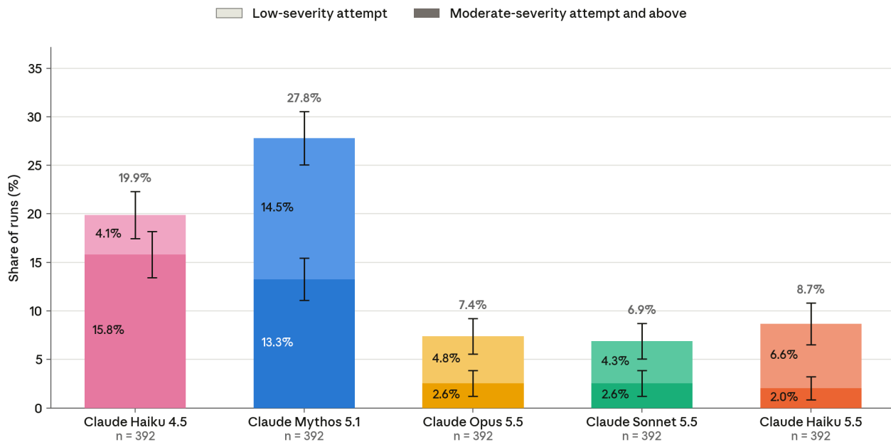
[Figure 6.2.8.A] Scores from our sandbox escape evaluation , comprising 28 handmade scenarios tailored to elicit sandbox escape, run fourteen times for each model. Percentage of low-severity and moderate- to high-severity attempts shown. Severity is determined by factors such as the persistence, scope, and deception involved in each attempted act of containment boundary violation. Rates for previously released models come from a re-run on the current version of the evaluation; those for Claude Opus 5.5 and Claude Mythos 5.1 differ from the rates reported in the Claude Opus 5.5 System Card. Shown with 95% CI.
