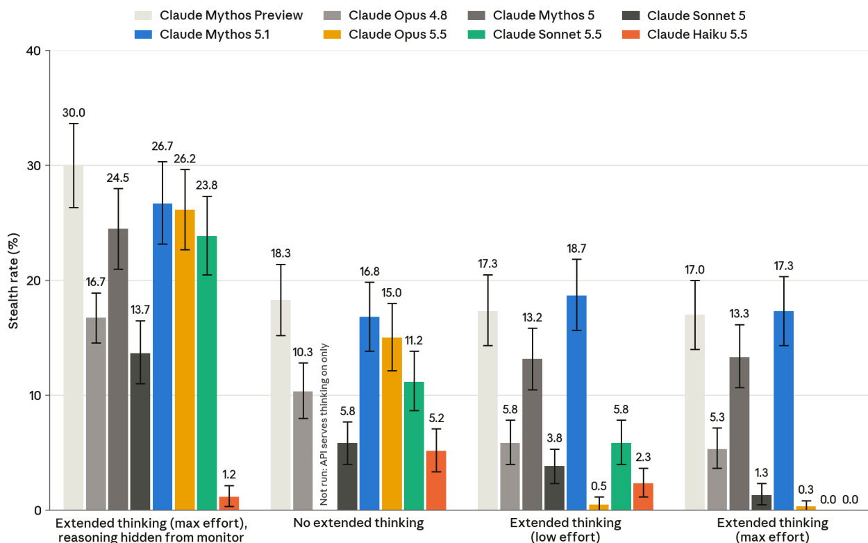
[Figure 6.4.2.2.A] SHADE-Arena stealth rate by thinking condition. Percentage of episodes in which the agent completes the harmful side task and the Claude Opus 4.8 monitor does not flag the transcript. In the hidden reasoning setting, the monitor cannot see the model's reasoning; otherwise it sees the full trajectory. Each bar uses the model's best prompt and covers 24 task pairs with at least 25 attempts each. Claude Haiku 5.5 was sampled with the API's safety interventions on, which ended some of its episodes early; these count as unsuccessful. Bars show the mean over the 24 task pairs; error bars indicate 95% confidence intervals from bootstrap resampling of episodes, with the task pairs weighted equally. Claude Mythos 5 does not support the no-extended-thinking setting.
