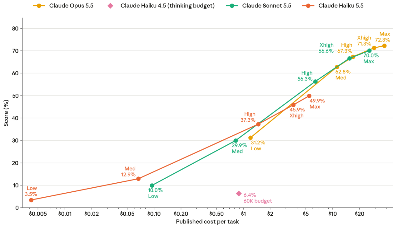
[Figure 8.8.3.A] WANDR soft F1 score versus average cost per task across reasoning effort levels at a 980k token task budget (log scale). Costs for Opus 5.5 and Sonnet 5.5 assume a perfect cache hit rate; Haiku 4.5 and 5.5 use list prices on recorded usage, with web search fees excluded. Claude Haiku 4.5 is shown at a 60K-token extended-thinking budget with 160K task budget.
