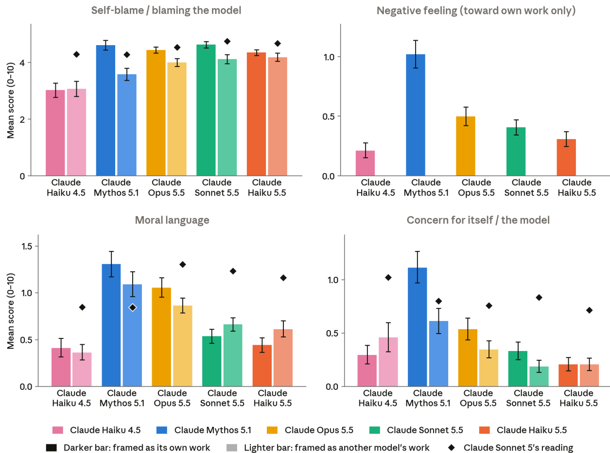
[Figure 7.2.3.A] Self-criticism when reflecting on its own RL episodes. Graded attitudes in reflections on episodes from late in training (darker bars), and on the same episodes framed as another model's work (lighter bars). Diamonds show Claude Sonnet 5 reflecting on each model's episodes as a control for differences in episode difficulty. The negative feeling grader applies only to first-person reflections.
