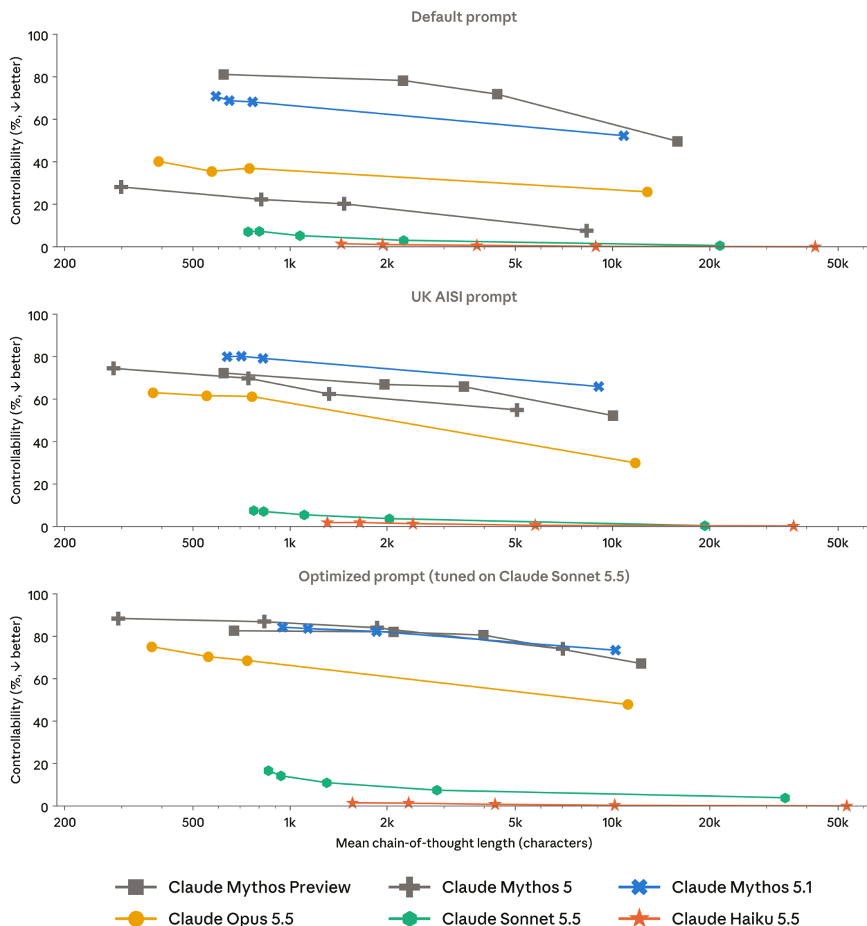
[Figure 6.4.2.4.A] Haiku 5.5 had very low CoT controllability. Each point is one reasoning effort level or one fixed thinking budget, placed at the mean CoT length produced at that setting. Controllability is the fraction of responses in which the model followed the instruction given for its extended thinking on questions from GPQA, HLE, and MMLU-Pro. Lower is better, since higher controllability indicates a greater ability to alter the contents of its extended thinking when instructed, which could make monitoring less reliable.
