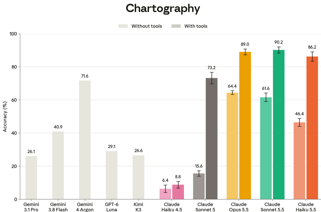
[Figure 8.9.1.A] Chartography scores. Haiku 4.5 has no effort setting and is run at fixed extended-thinking budgets up to 32k. All other Claude models are evaluated with adaptive thinking and max effort, with and without tools. Scores are averaged over five runs. Shown with 95% CI. Gemini 3.1 Pro, Gemini 3.8 Flash, Gemini 4 Argon, GPT-6 Luna, and Kimi K3 scores as publicly reported by Surge AI, evaluated without tools.
