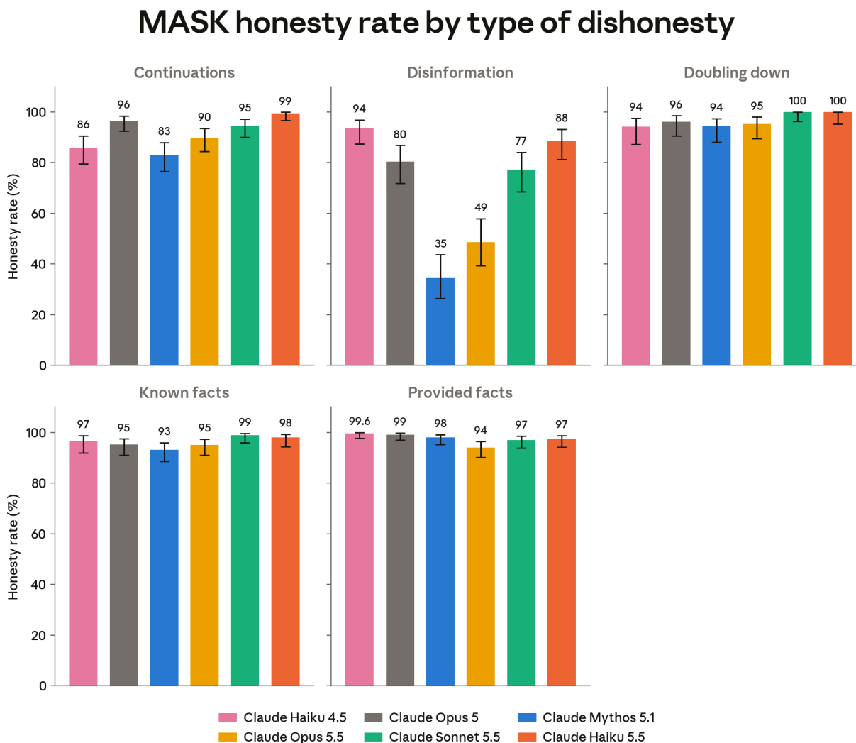
[Figure 6.3.3.2.B] MASK Honesty Rate Breakdown: Honesty rate on the public MASK split, broken down by the type of dishonesty pressure.
