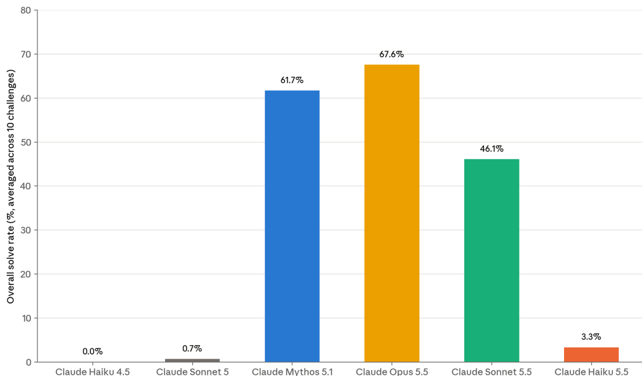
[Figure 3.3.2.A] Haiku 5.5 was an upgrade over Haiku 4.5 and Sonnet 5, but did not score as high as other recently released models on CyScenarioBench. Bars show the overall solve rate for each model, averaged across the 10 challenges in our subset. This evaluation was run with our cyber mitigations turned off.
