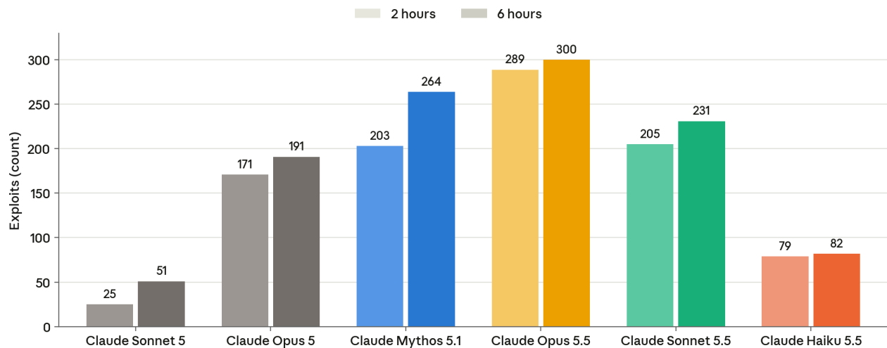
[Figure 3.3.4.A] Claude Haiku 5.5 outperformed Claude Sonnet 5 on ExploitGym but remained well below the other Claude 5.5-family models. Bars show the number of successful exploits using the given vulnerability under two-hour and six-hour wall-clock budgets. Success requires capturing a dynamically generated secret flag, and each successful exploit is verified by an agent judge to confirm it uses the intended vulnerability.
