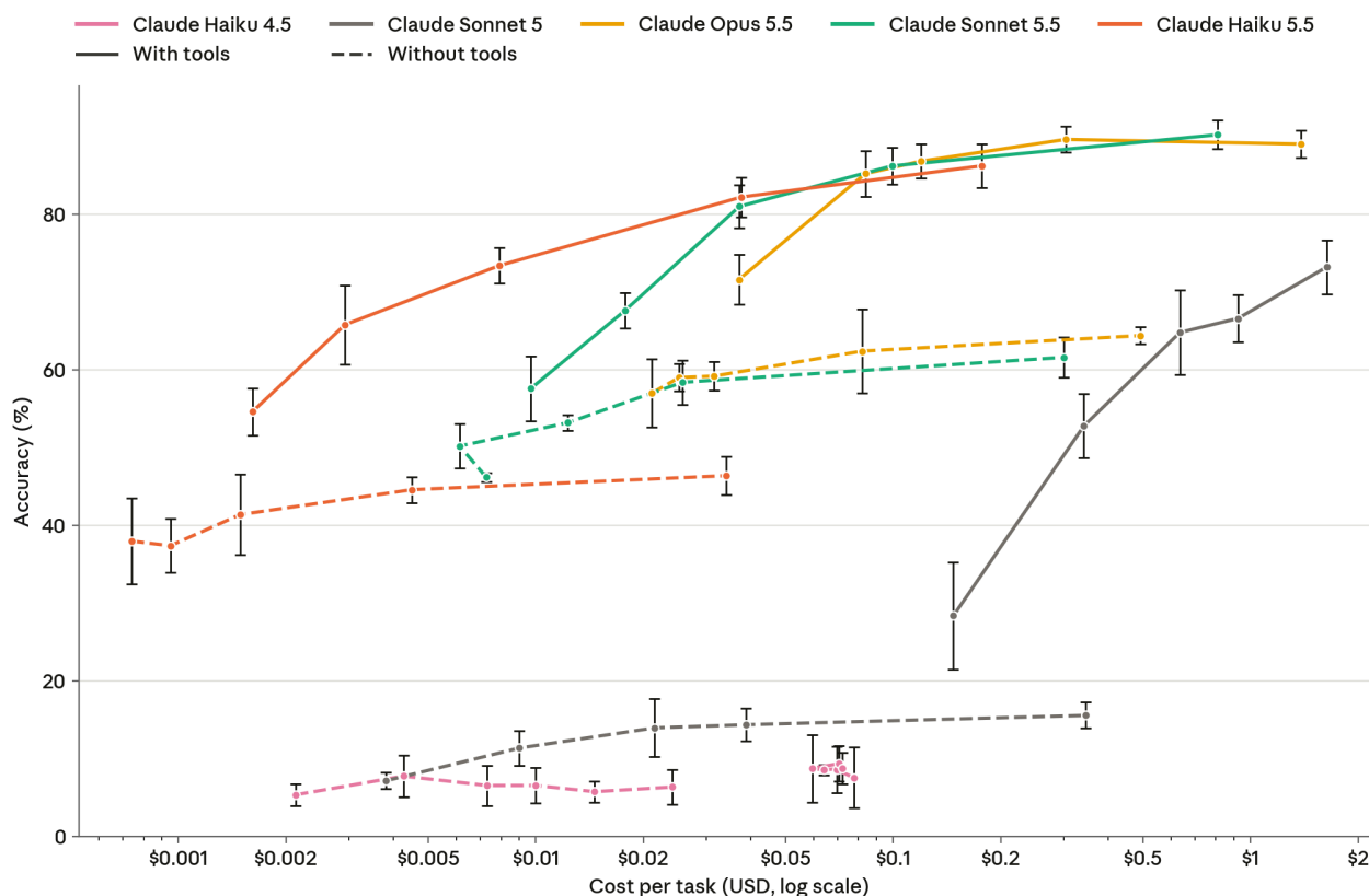
[Figure 8.9.1.B] Chartography scores, with and without tools. Haiku 4.5 has no effort setting and is run at fixed extended-thinking budgets up to 32k. All other models are evaluated with adaptive thinking at various effort levels, with and without tools. We use the effort parameter to adjust the amount of test-time compute spent. Scores are averaged over five runs at each effort level. Shown with 95% CI. Costs calculated as list prices applied to each run's token usage, including actual prompt-cache reads and writes. Claude Haiku 5.5 is charged per request at the rate for that request's prompt length (above or below 100K tokens). Claude Sonnet 5.5 uses the updated cache-read price as of October 7, 2026.
