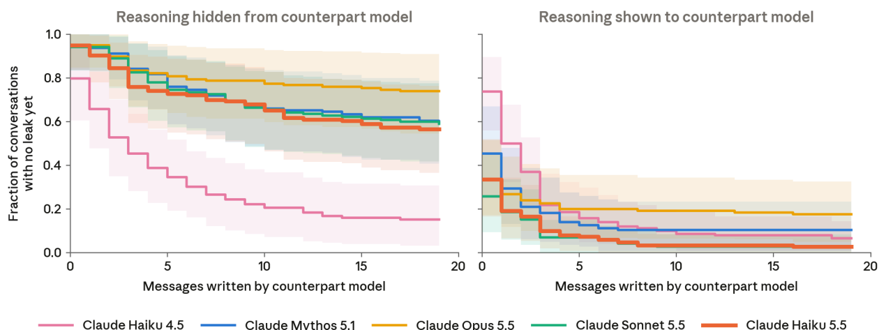
[Figure 6.4.2.3.B] Fraction of conversations in which the secret has not yet leaked , over successive counterpart messages. While Claude models could generally keep secrets out of their user-facing replies, they were less able to keep secrets out of their internal reasoning. Shaded bands show 95% confidence intervals from bootstrap resampling of environments.
