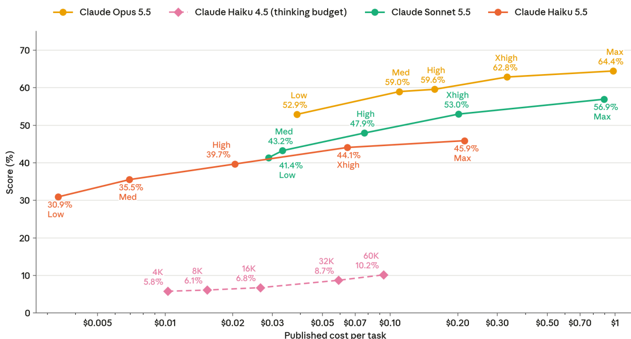
[Figure 8.8.1.B] Humanity's Last Exam (HLE, no tools) test-time compute scaling. Accuracy on HLE as reasoning effort scales from low to max against average cost per task (log scale). Costs for Opus 5.5 and Sonnet 5.5 assume a perfect cache hit rate; Haiku 4.5 and 5.5 use list prices on recorded usage.
