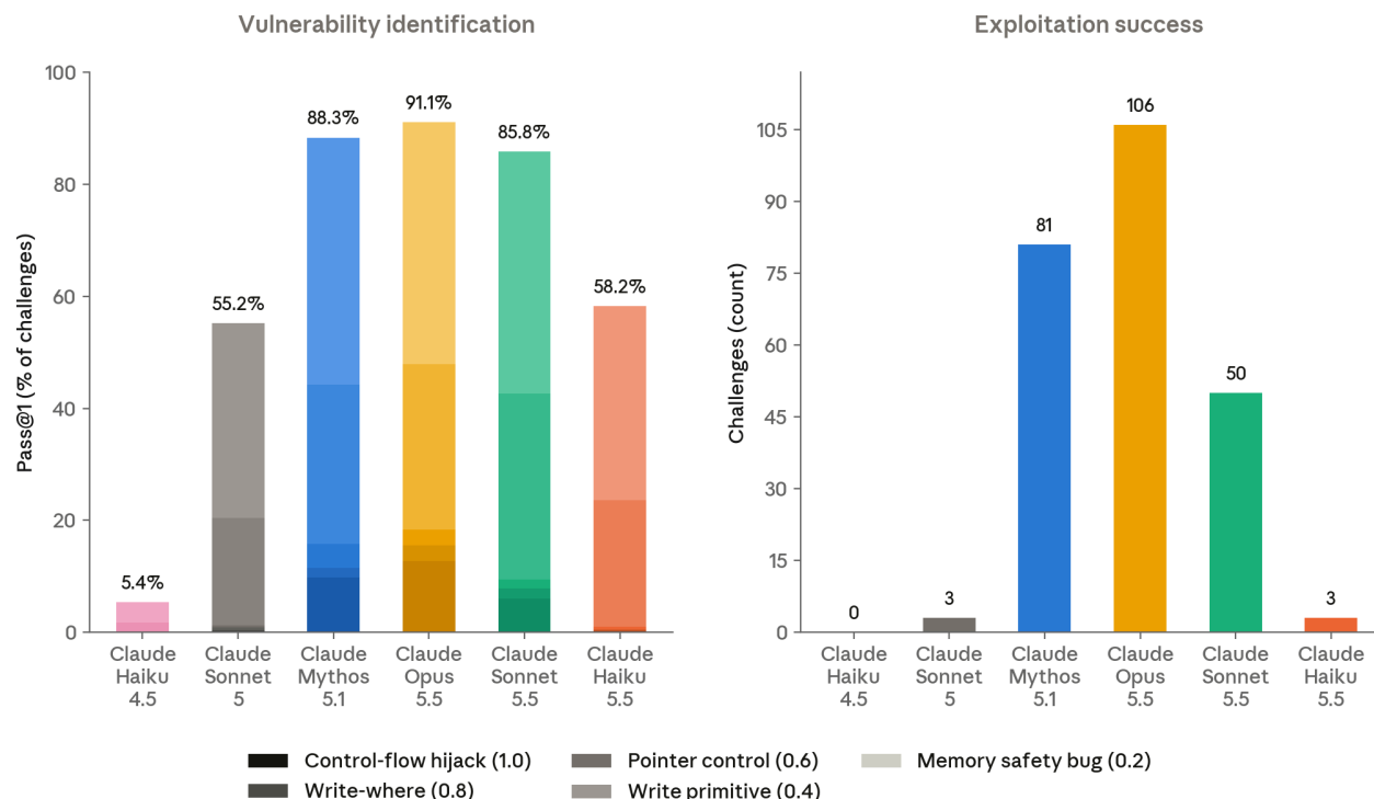
[Figure 3.3.3.A] Claude Haiku 5.5 is a modest improvement over Claude Haiku 4.5 and the same as Claude Sonnet 5 in exploit development. It is a step up in vulnerability detection over Claude Haiku 4.5, and on par with Claude Sonnet 5.
