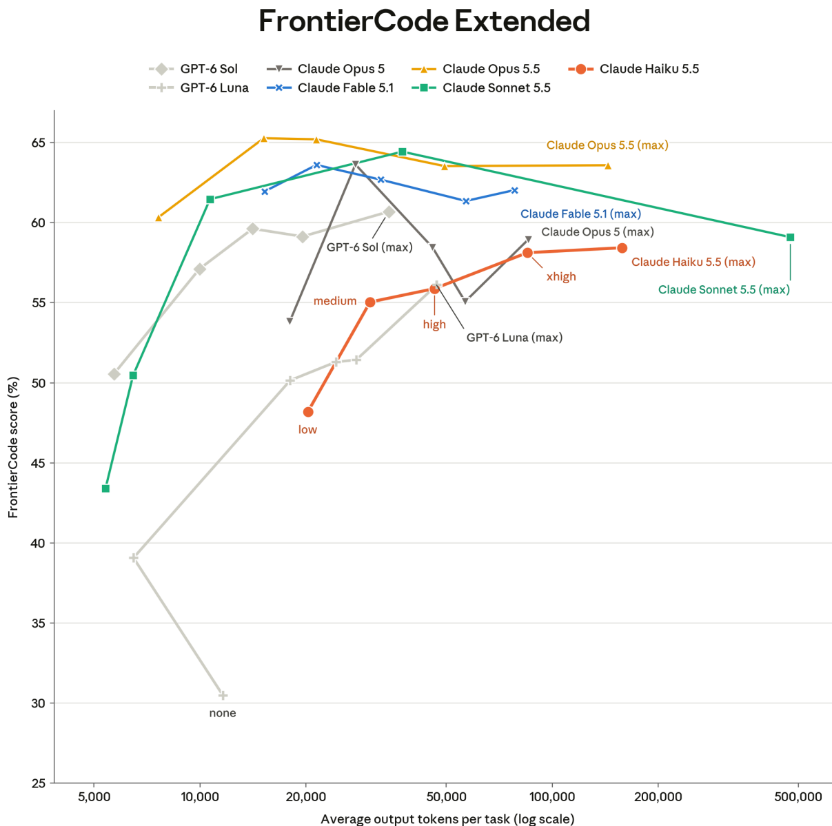
[Figure 8.3.B] FrontierCode Extended score versus average output tokens per task across reasoning effort levels ( low , medium , high , xhigh and max ; GPT-6 Luna also at none ). Cognition ran the evaluation for every model shown and reported the results; Claude models were run in Claude Code and GPT models were run in Codex. Cognition's result files report token counts for every model and no cost for Claude Haiku 5.5, so the x-axis shows average output tokens per task, on a logarithmic scale. Each Claude Haiku 5.5 point is labeled with its effort level (its max point with the model's name). Every other model is labeled with its name at its max point, and GPT-6 Luna's none point is also labeled with its effort level. Each line joins a model's points in order of effort. The result files carry no uncertainty intervals, so none are shown. Note that the y-axis begins at 25%, not at zero, so differences between points are visually magnified.
