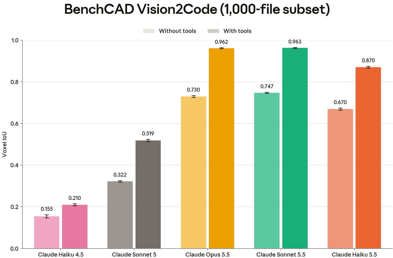
[Figure 8.9.2.A] BenchCAD Vision2Code subset scores. Haiku 4.5 has no effort setting and is run at fixed extended-thinking budgets up to 32k. All other Claude models are evaluated with adaptive thinking and max effort, with and without tools. Scores are averaged over five runs and shown with 95% CI.
