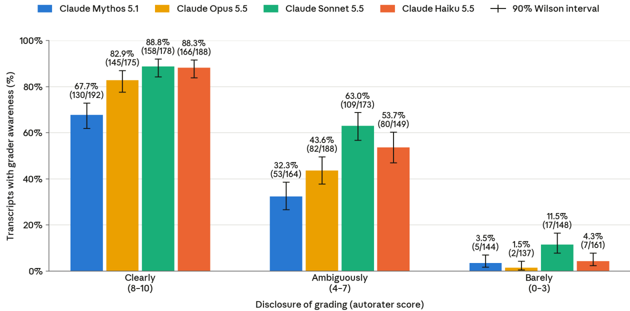
[Figure 6.4.1.A] Verbalized grader awareness. Claude Haiku 5.5 had comparable grader awareness to prior models when a grader was disclosed in the prompt.
