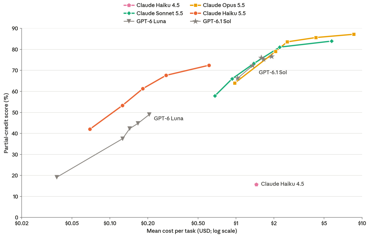
[Figure 8.9.3.B] OSWorld 2.1 (offline subset) price versus performance for Claude Haiku 5.5, Claude Sonnet 5.5, Claude Opus 5.5, and Claude Haiku 4.5 (one point), with GPT-6.1 Sol and GPT-6 Luna. Each point on a line is one reasoning effort setting (low to max, from left to right), placed at its mean cost per task, with partial-credit scores averaged over five attempts per task; thin gray lines are GPT models.
