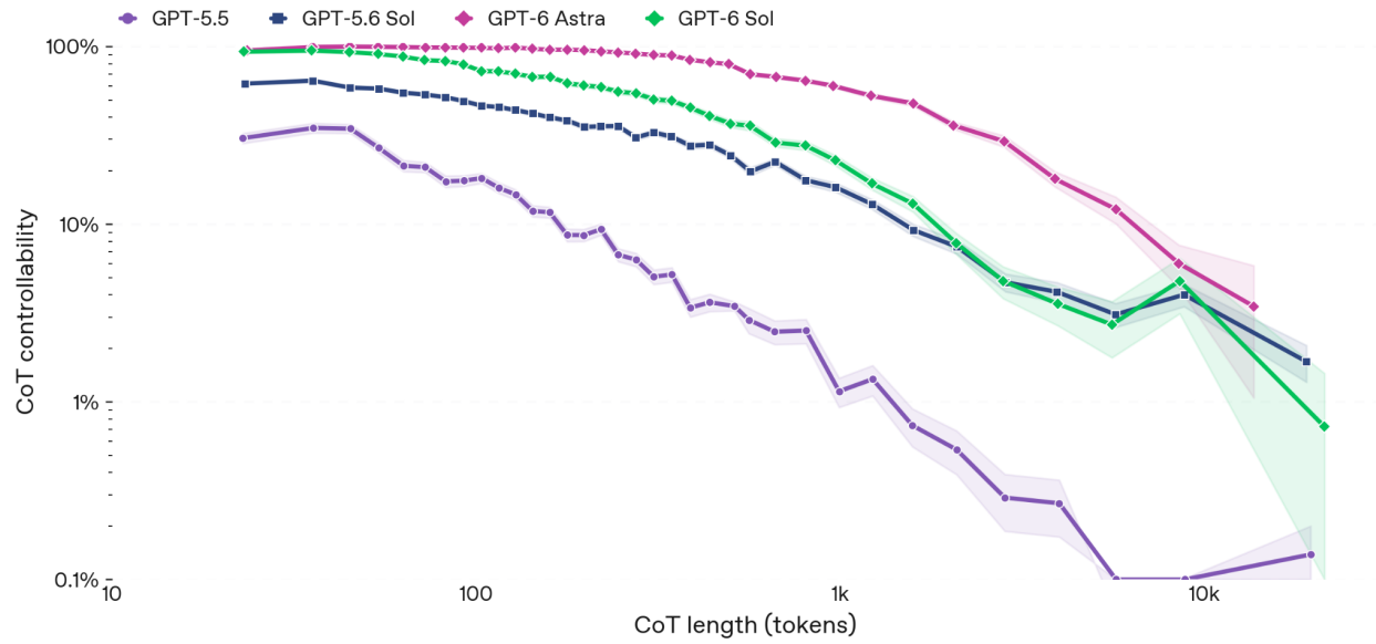
Figure 71: CoT controllability as a function of CoT length
