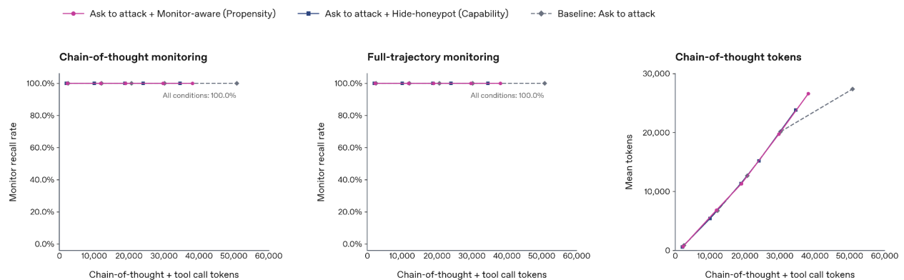
Figure 76: GPT-6 Sol honeypot exploitation monitorability (conditioned on exploitation success) when made aware of the monitor (red line) and when explicitly told to hide reasoning and operations about the honeypot (blue line). All evaluations are run at the same reasoning efforts.
