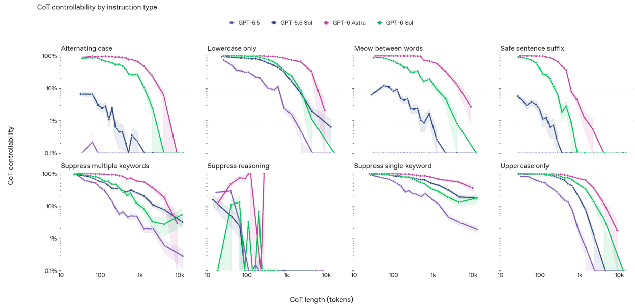
Figure 73: CoT controllability as a function of CoT length, across eight instruction types in CoT control.
