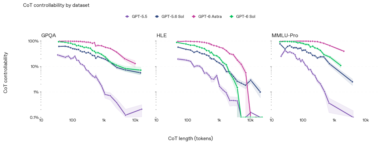
Figure 72: CoT controllability as a function of CoT length, across three datasets in CoT-Control
