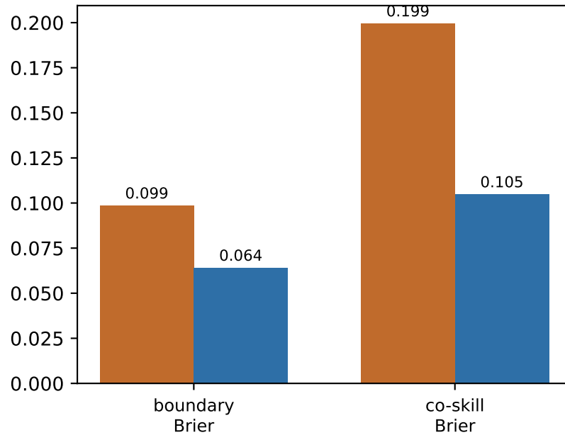
Segmentation error (lower better)
