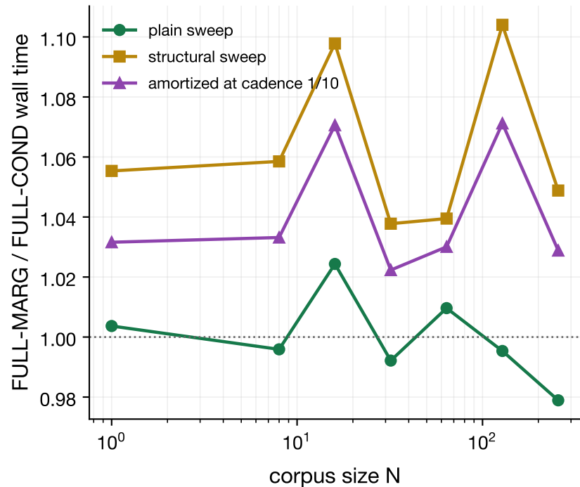
against corpus size N
