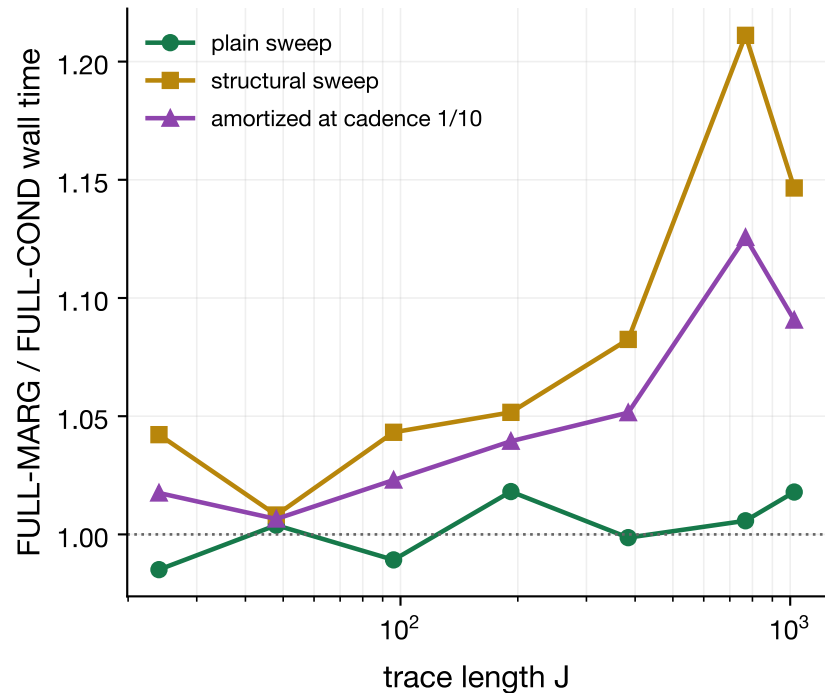
against trace length J
