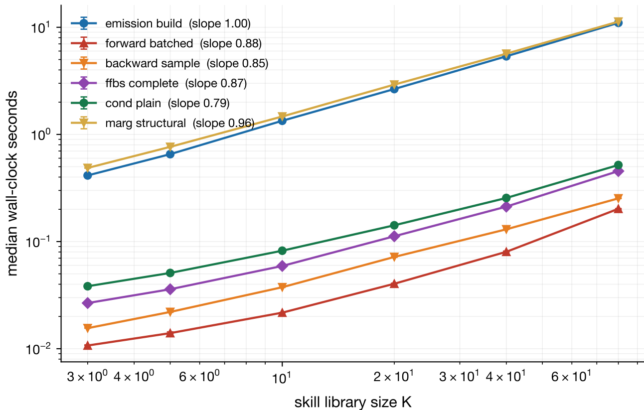
Scaling in the skill library ( N=32 , J=128 , A=20 , D in [3,12] )
