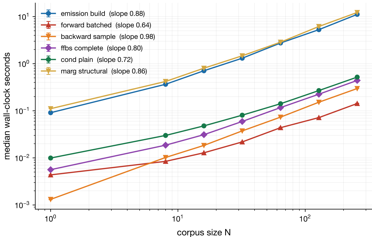
Scaling in corpus size (J=128, K=10, A=20, D in [3,12])
