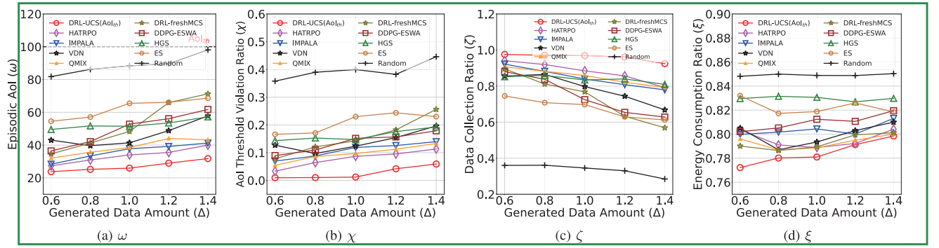
Fig. 11. Impact of generated data amount in a timeslot (Beijing).
