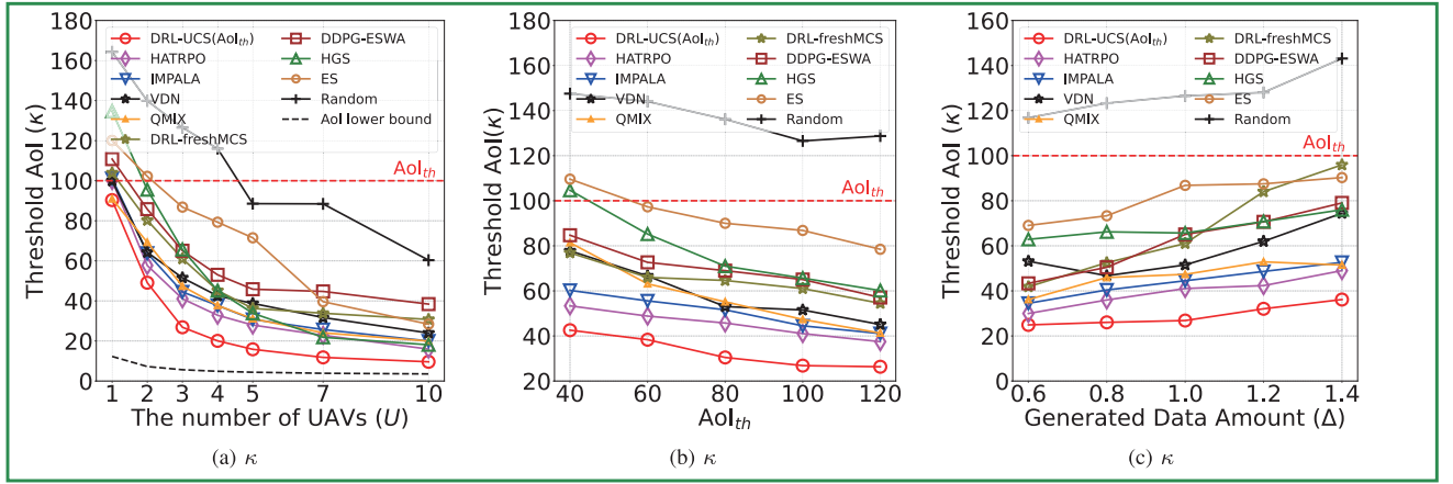
Fig. 4. Threshold AoI w.r.t. U , AoI_{th} and \Delta (Beijing).
