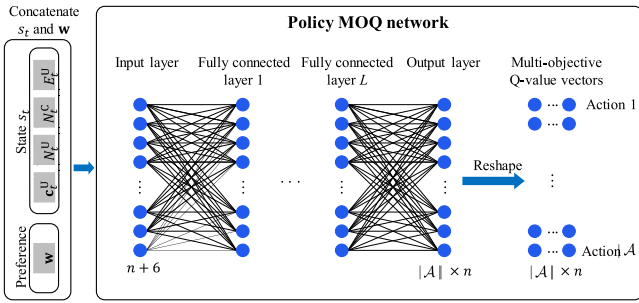
Fig. 3. Network architecture.
