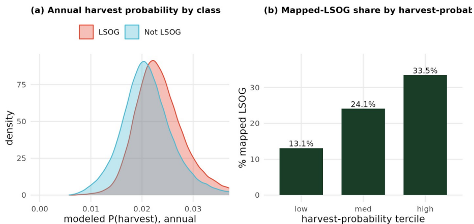
Figure S5. (a) Annual harvest probability (HCS v5 CONUS model: clearcut plus partial) for mapped-LSOG versus non-LSOG pixels over the Maine AOI ( n = 3.8 million), and (b) the mapped-LSOG share by harvest-probability tercile. Contrary to a simple accessibility intuition, mapped LSOG sits where modeled harvest probability is highest: the LSOG share rises from 13% in the lowest harvest-probability tercile to 34% in the highest, and LSOG pixels carry higher mean annual harvest probability (0.024 versus 0.021) and disturbance probability (0.128 versus 0.111) than non-LSOG. The likely mechanism is that the structure that reads as LSOG (large trees, high stocking) is also what makes a stand merchantable, so the mapped resource is not shielded by low harvest pressure.
