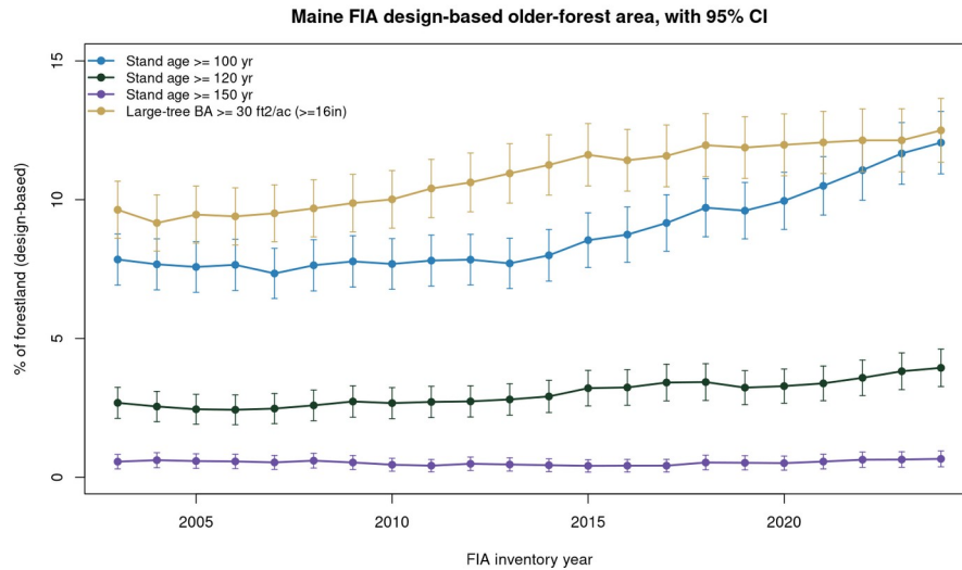
Fig. 2. FIA design-based older-forest area (stand age \geq 120 yr) for Maine, 2003-2024, with 95% confidence intervals. The stock rises while total forestland area is flat.
