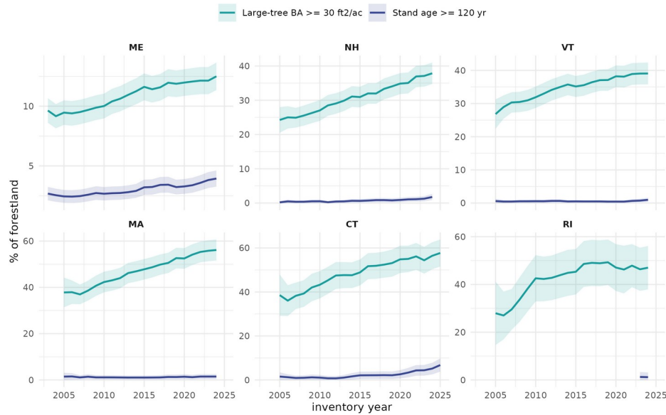
Fig. 6. Design-based older-forest area for the six New England states by stand age \geq 120 yr and large-tree basal area, with 95% confidence bands. Both measures are stable to increasing in every state; the gap between them widens from north to south. The Rhode Island age trend is unestimable from its sparse plot panel, so its structural measure is the reliable one there.
