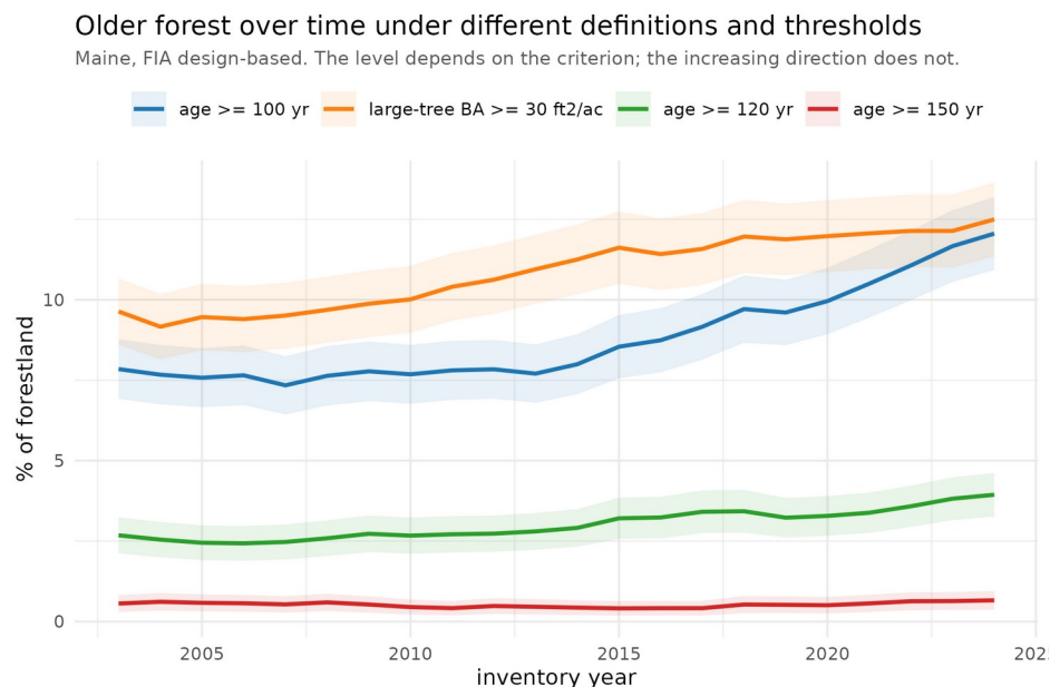
Figure S4. Maine older forest over time (FIA design-based) under four ground definitions: stand age \geq 100, \geq 120, and \geq 150 yr, and large-tree basal area \geq 30 ft-sq/ac, each with a 95% band. The level depends on the criterion, but every definition increases over 2003-2024.
