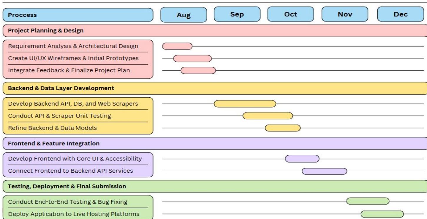
Gantt Chart
