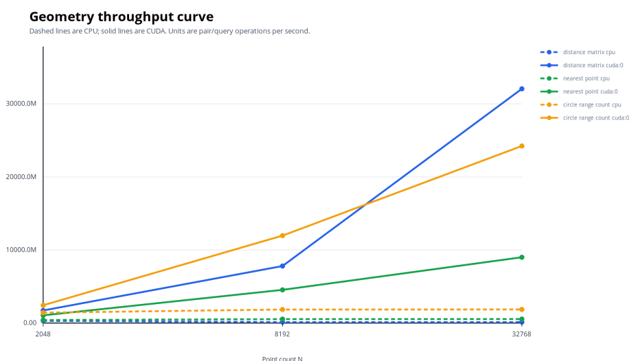
Figure 5.8: 几何算法吞吐量曲线 (Throughput curve)
