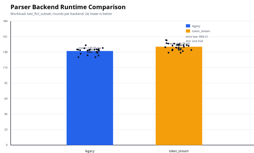
Figure 5.2: Parser backend 耗时对比 (Timing comparison between parser backends)
