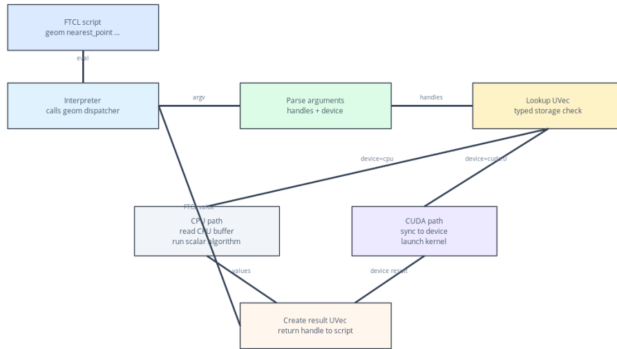
geom command execution flow Example: geom nearest_point $dataset $queries cuda:0
