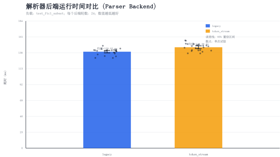
图 5.2: Parser backend 耗时对比 (Timing comparison between parser backends)
