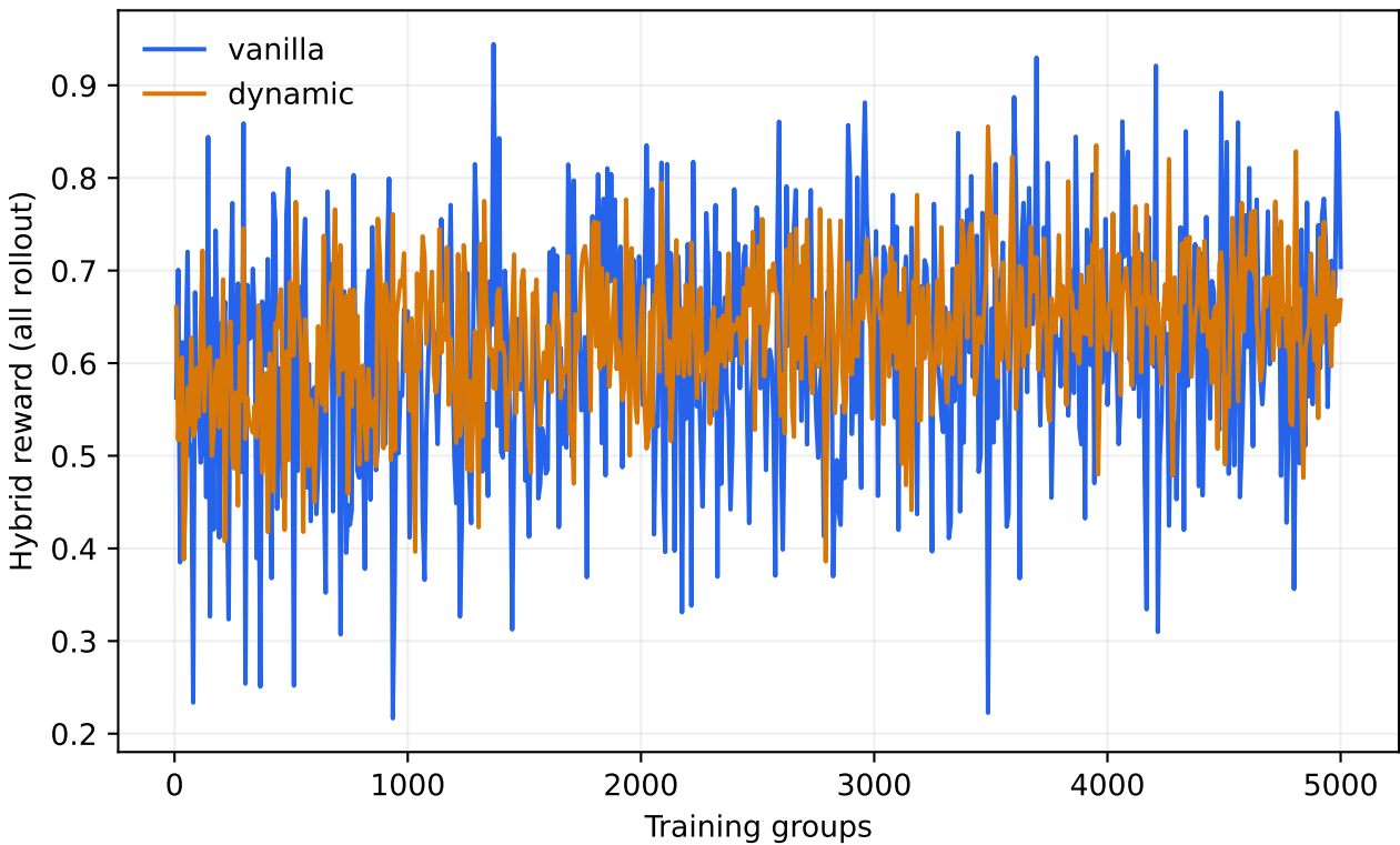
FORMAL · reward
